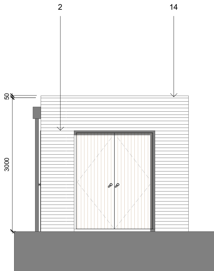
Front Elevation 1 : 50
