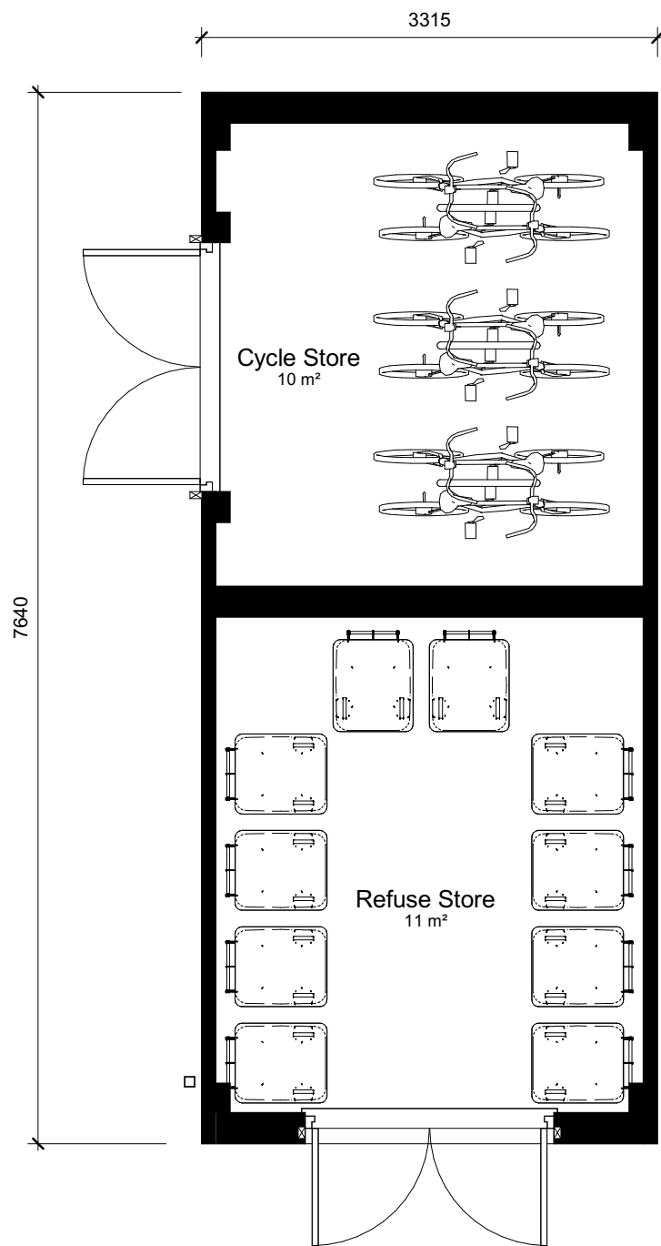
Ground Plan 1 : 50
