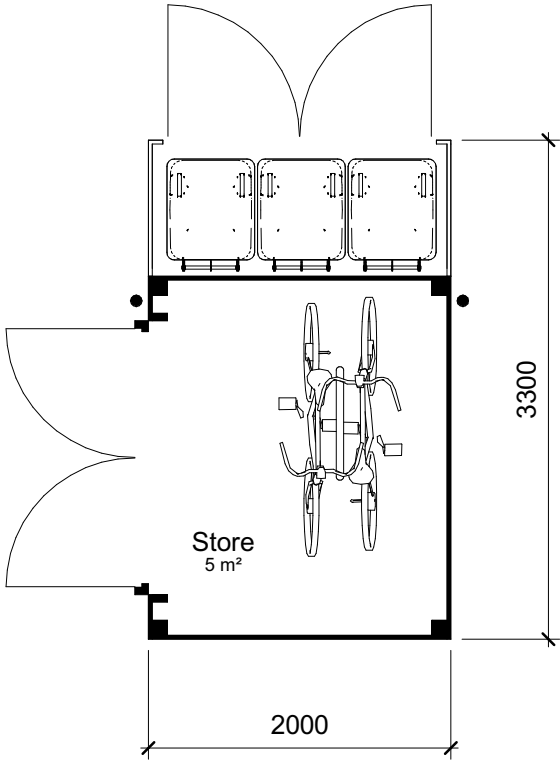
Ground Plan 1 : 50
