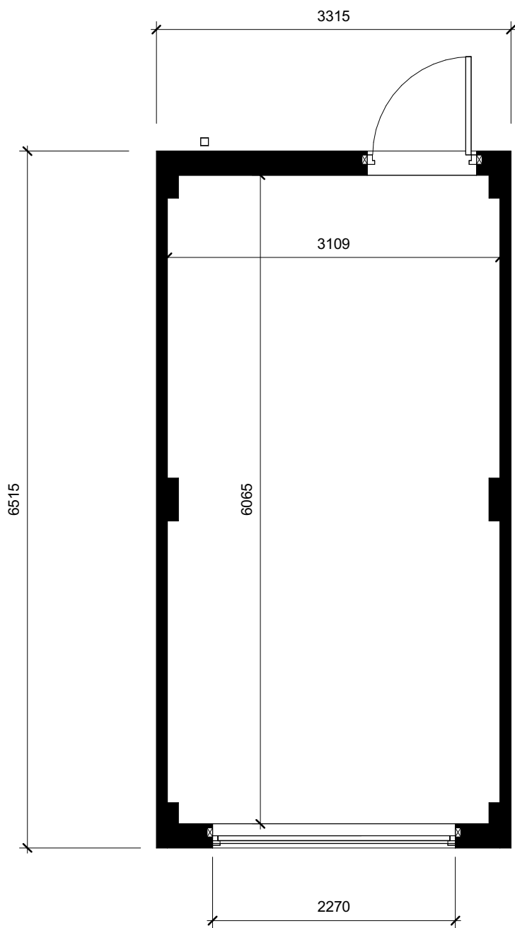
Ground Plan 1 : 50
