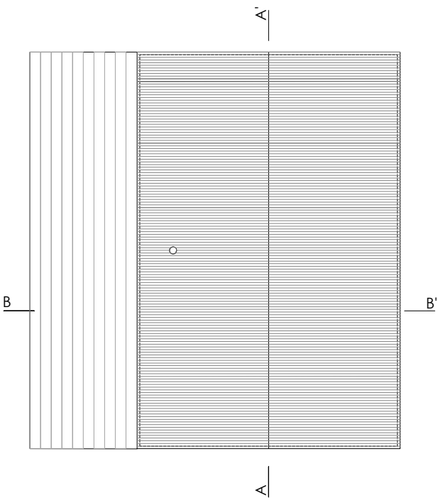
ROOF PLAN
