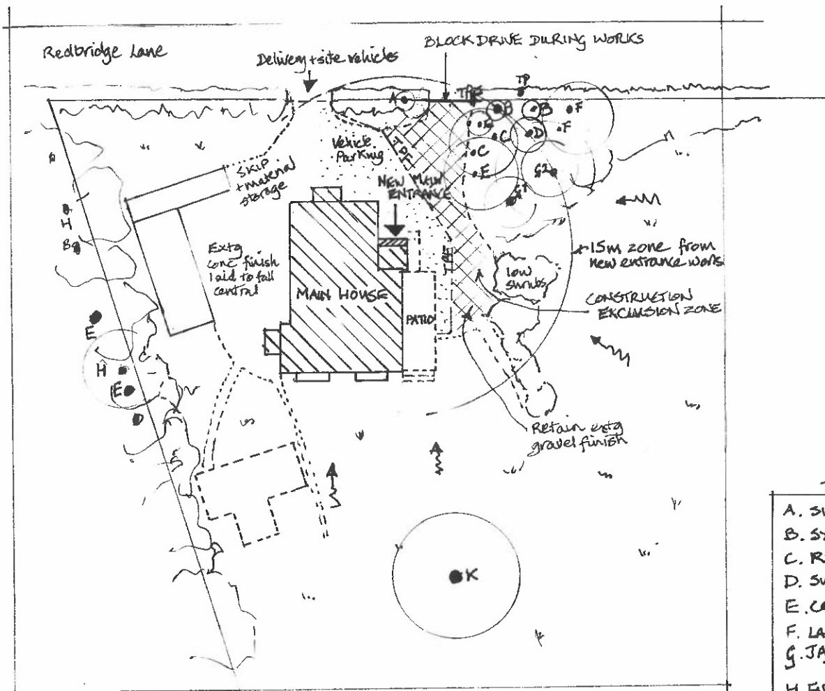
PART SITE PLAN
