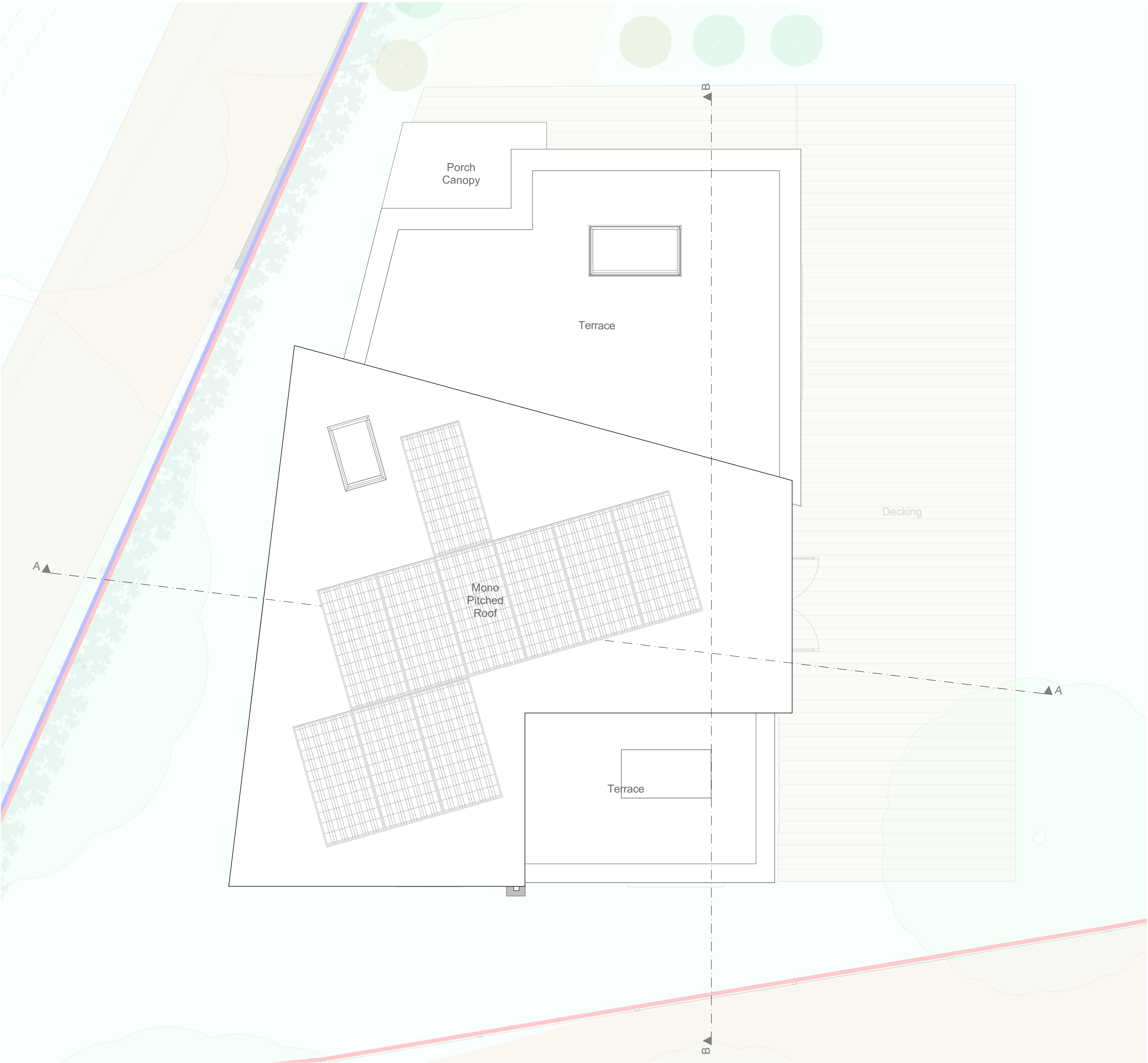
Proposed Roof Plan
