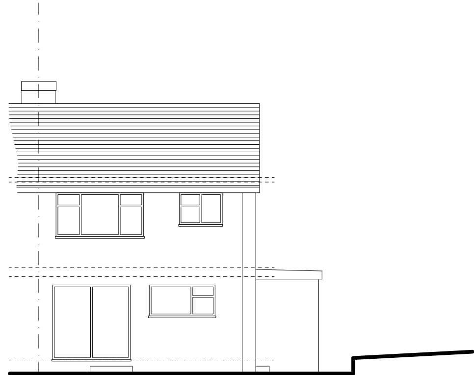
Rear Elevation (South)
