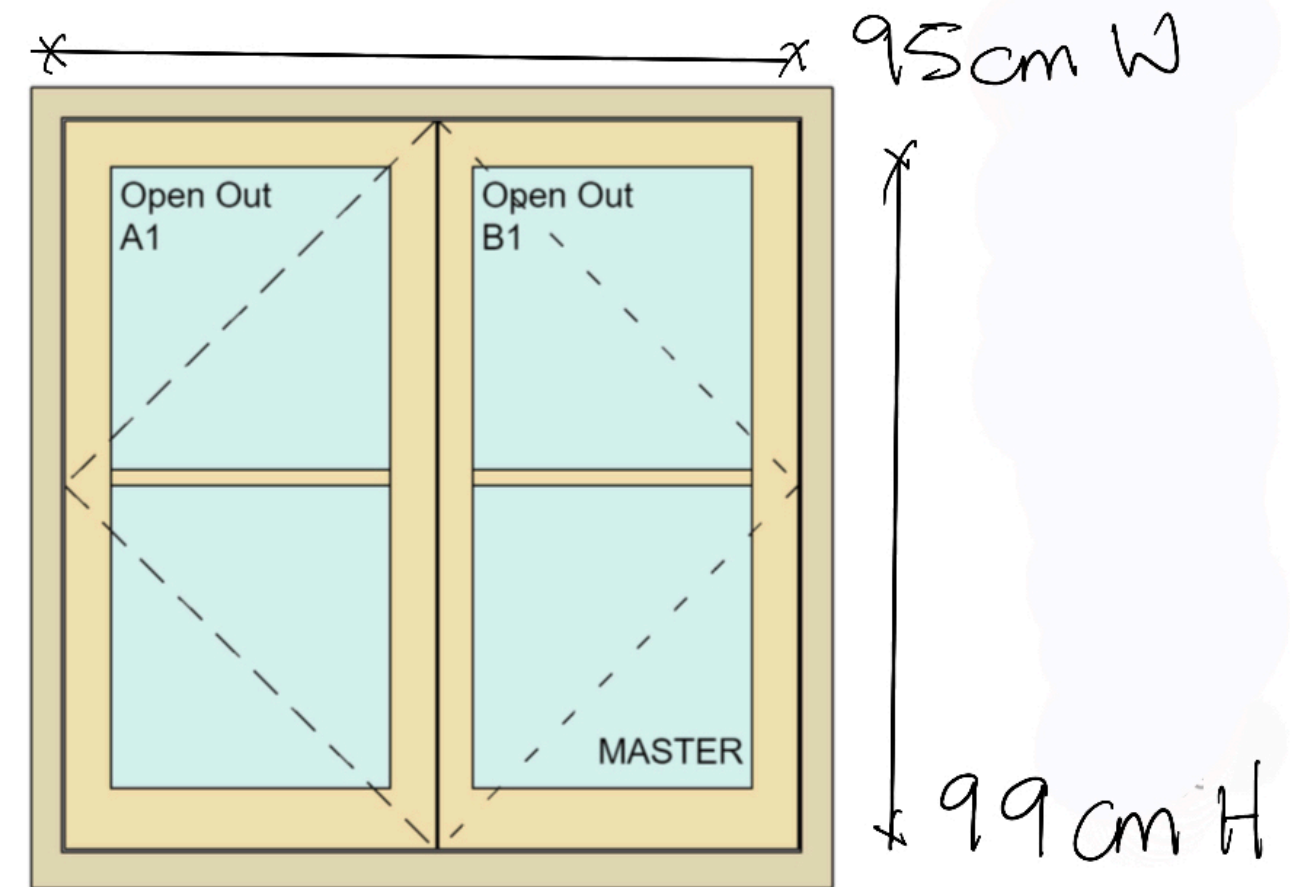
ITEM 10 - Ground Floor Front Elevation Dining area
