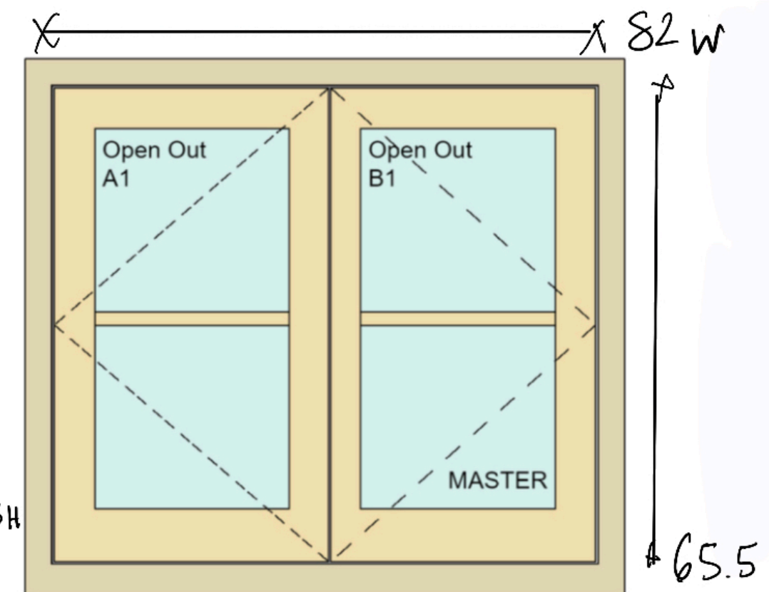
ITEM 13 - Ground Floor RHS Elevation Kitchen RH
