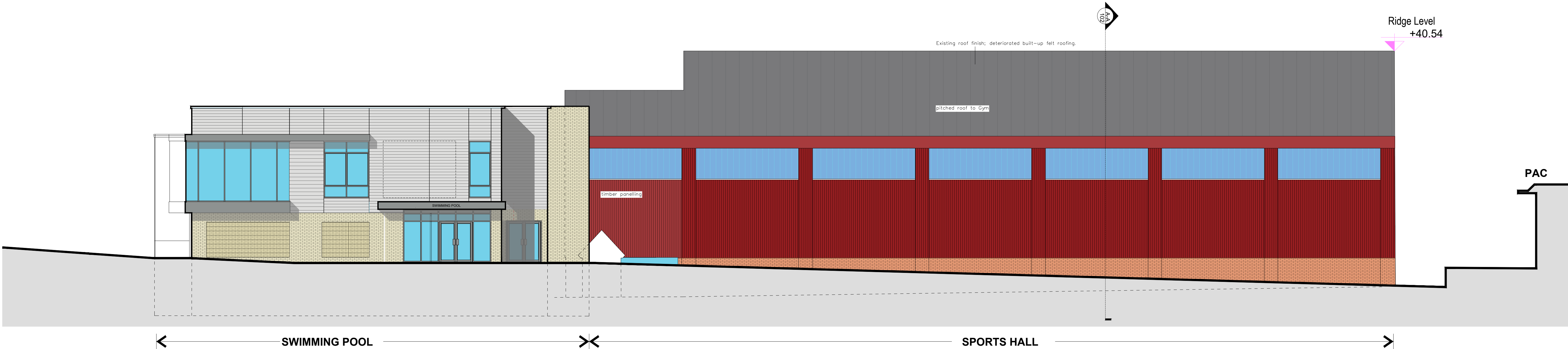
CONTEXTUAL ELEVATION NORTHERN - EXISTING Scale 1:100
