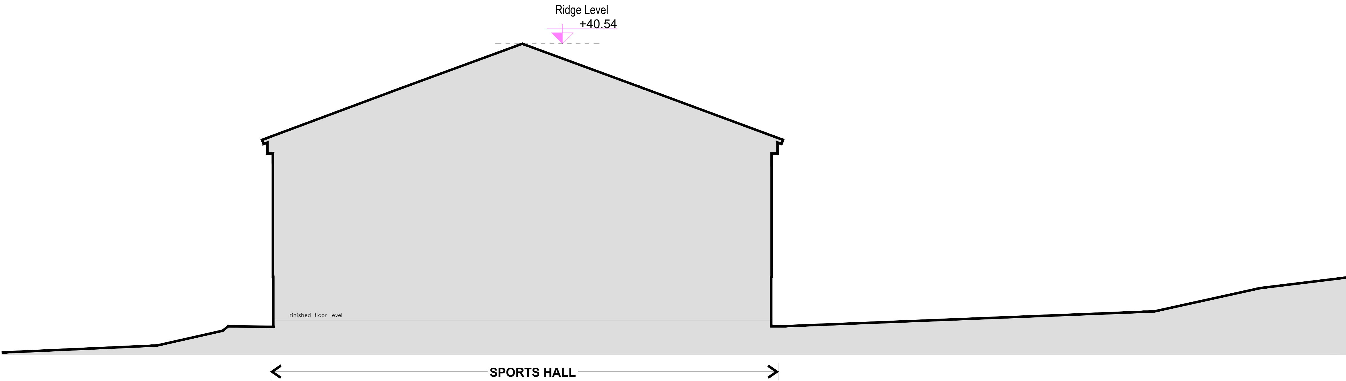
SECTION A-A - EXISTING Scale 1:100
