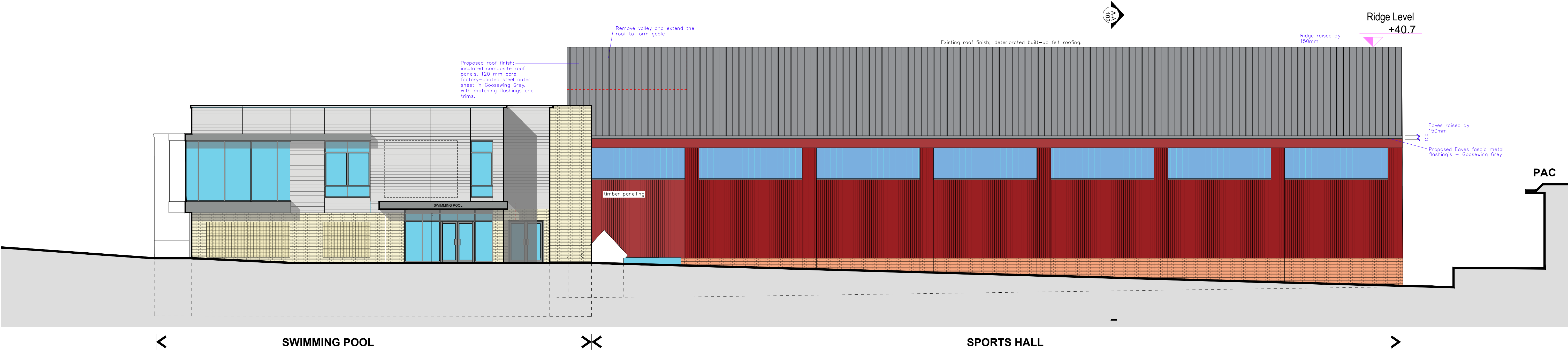
CONTEXTUAL ELEVATION NORTHERN - PROPOSED Scale 1:100
