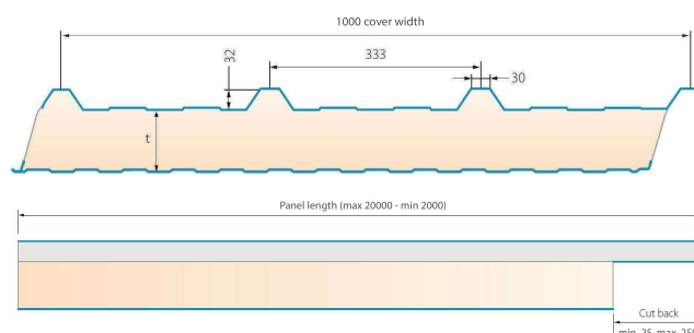
Figure 1. Trisomet® cross section and cut back
