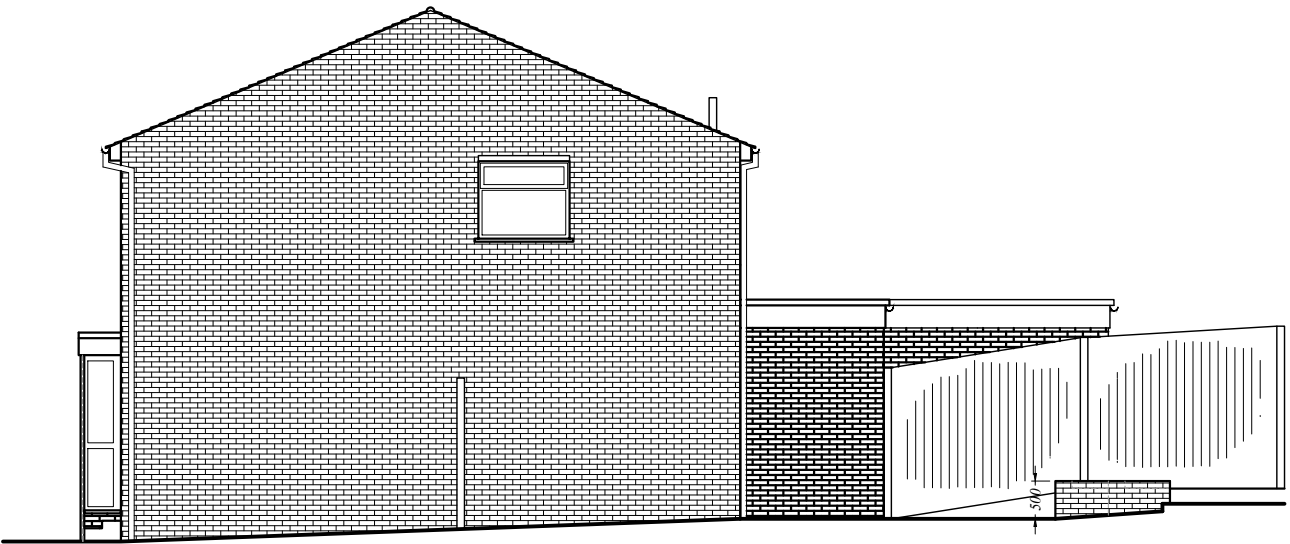
Side Elevation
