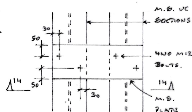
DETAIL 15.15
