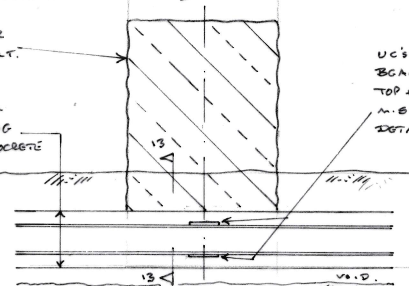
DETAIL 12-12
