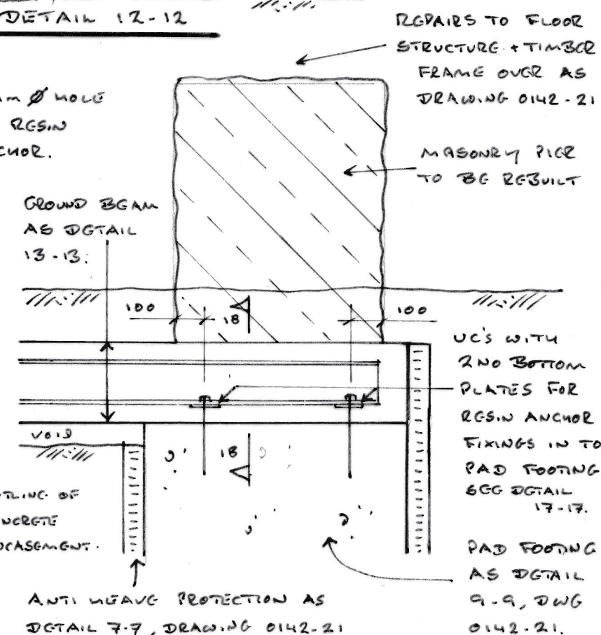
DETAIL 16-16
