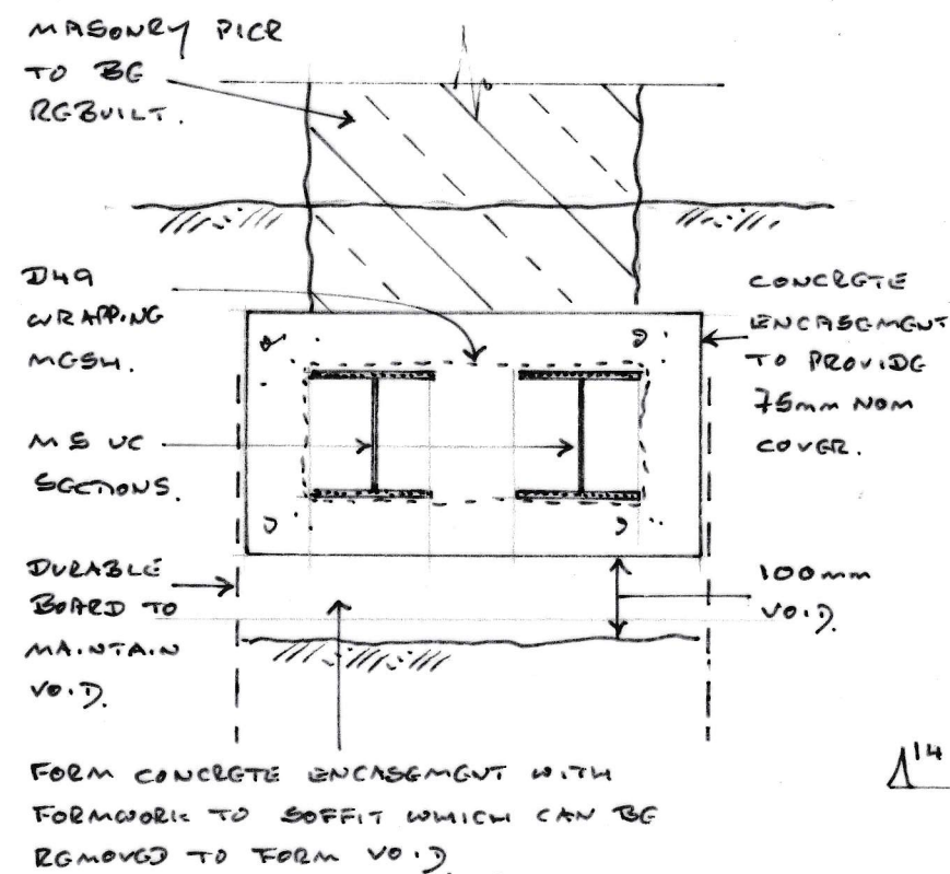
DETAIL 13-13
