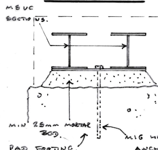
DETAIL 18-18
