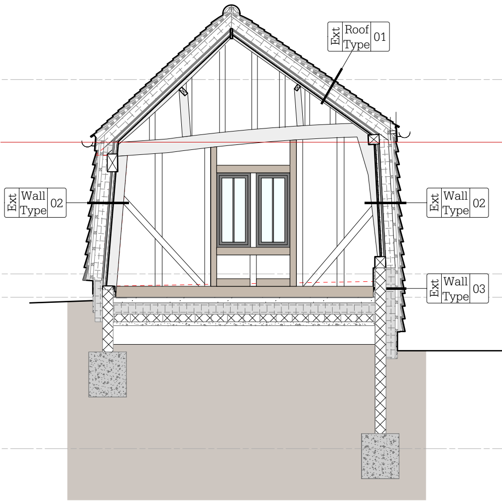
3 - Section B
