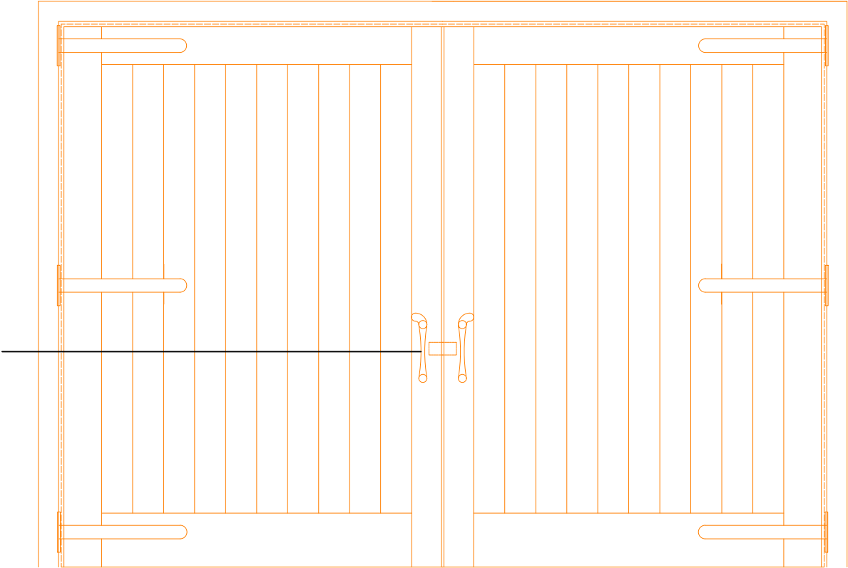
Elevation - External @ 1:20
