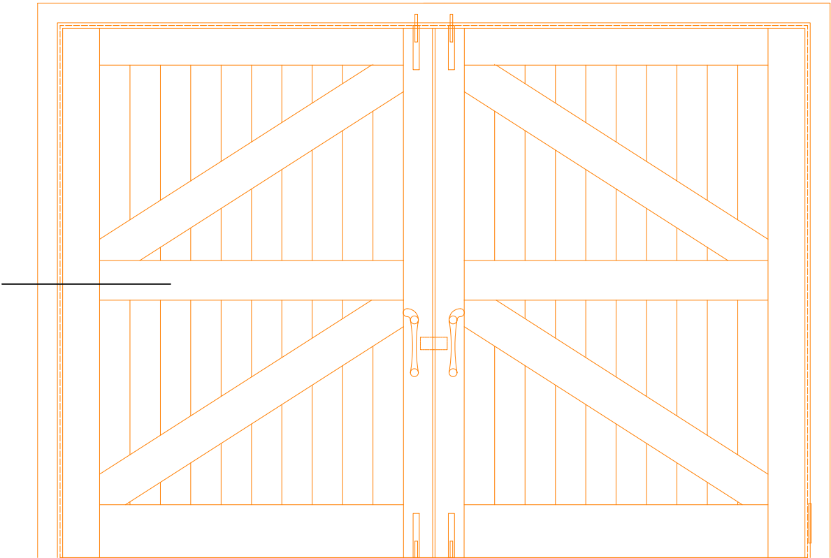
Elevation - Internal @ 1:20
