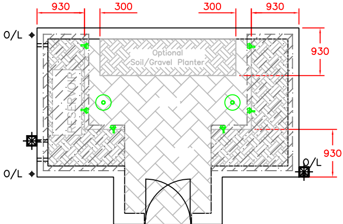
Floor layout for "General Grower" benching.
