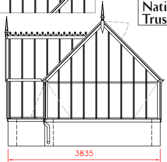
GABLE ELEVATION
