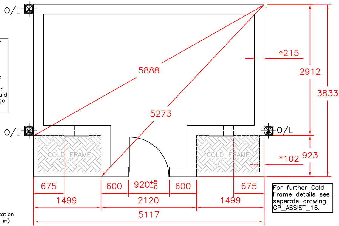
GROUND PLAN.
