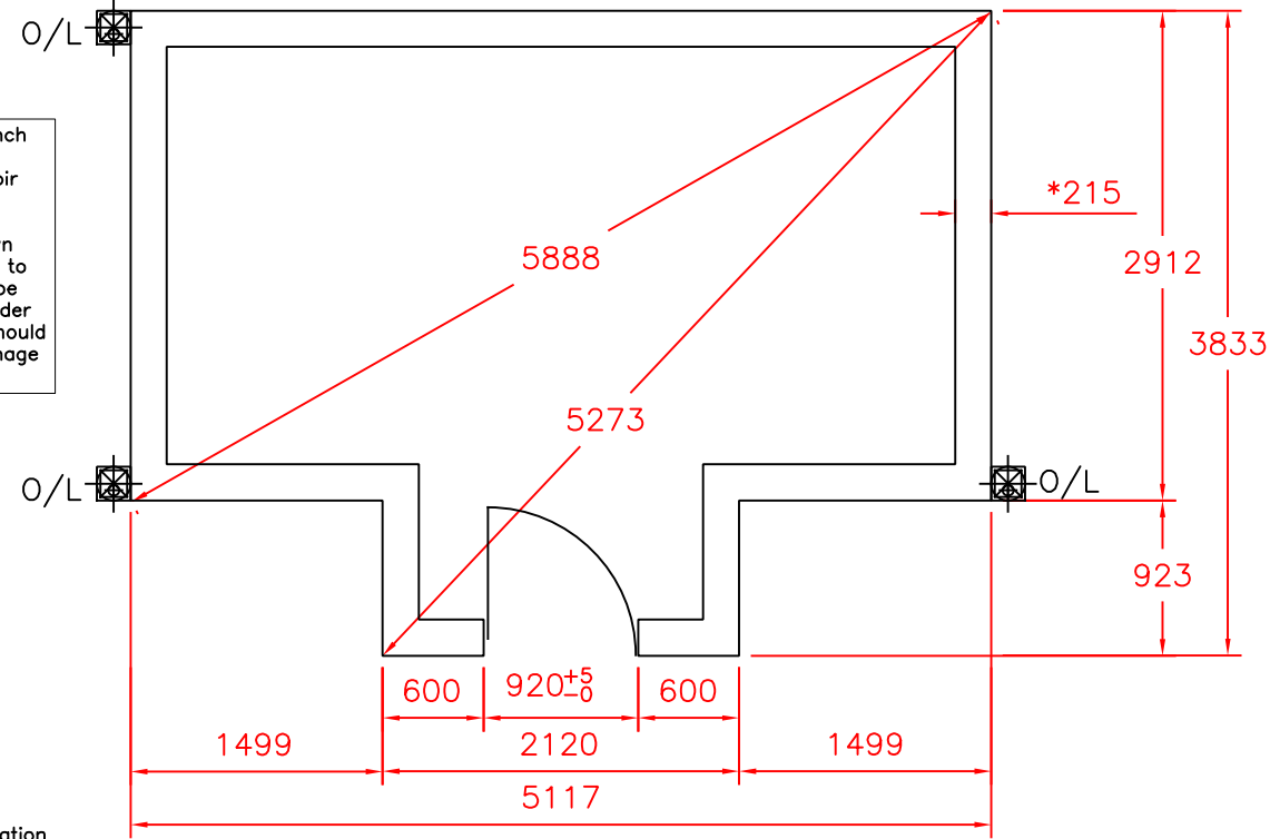
GROUND PLAN.
