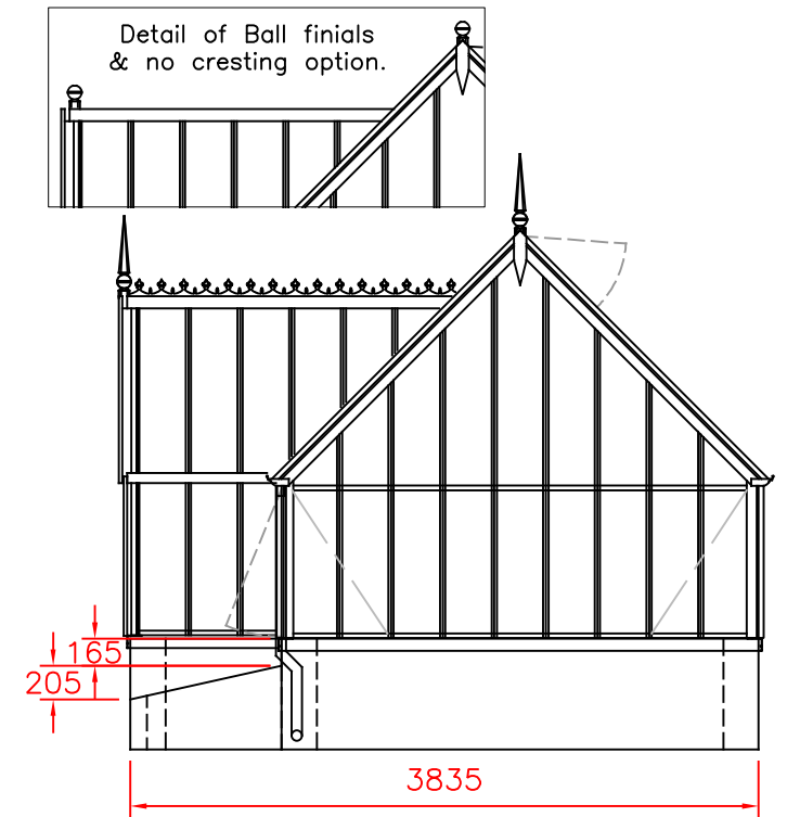
GABLE ELEVATION
