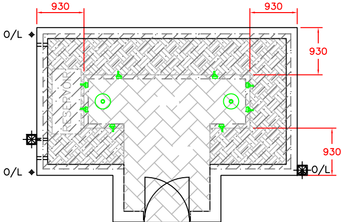
Floor layout for "Plantsman" benching.
