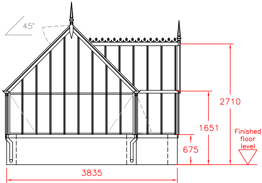
GABLE ELEVATION
