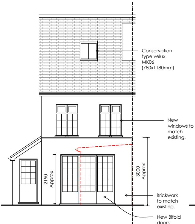
Proposed Rear Elevation Scale 1/100@A3
