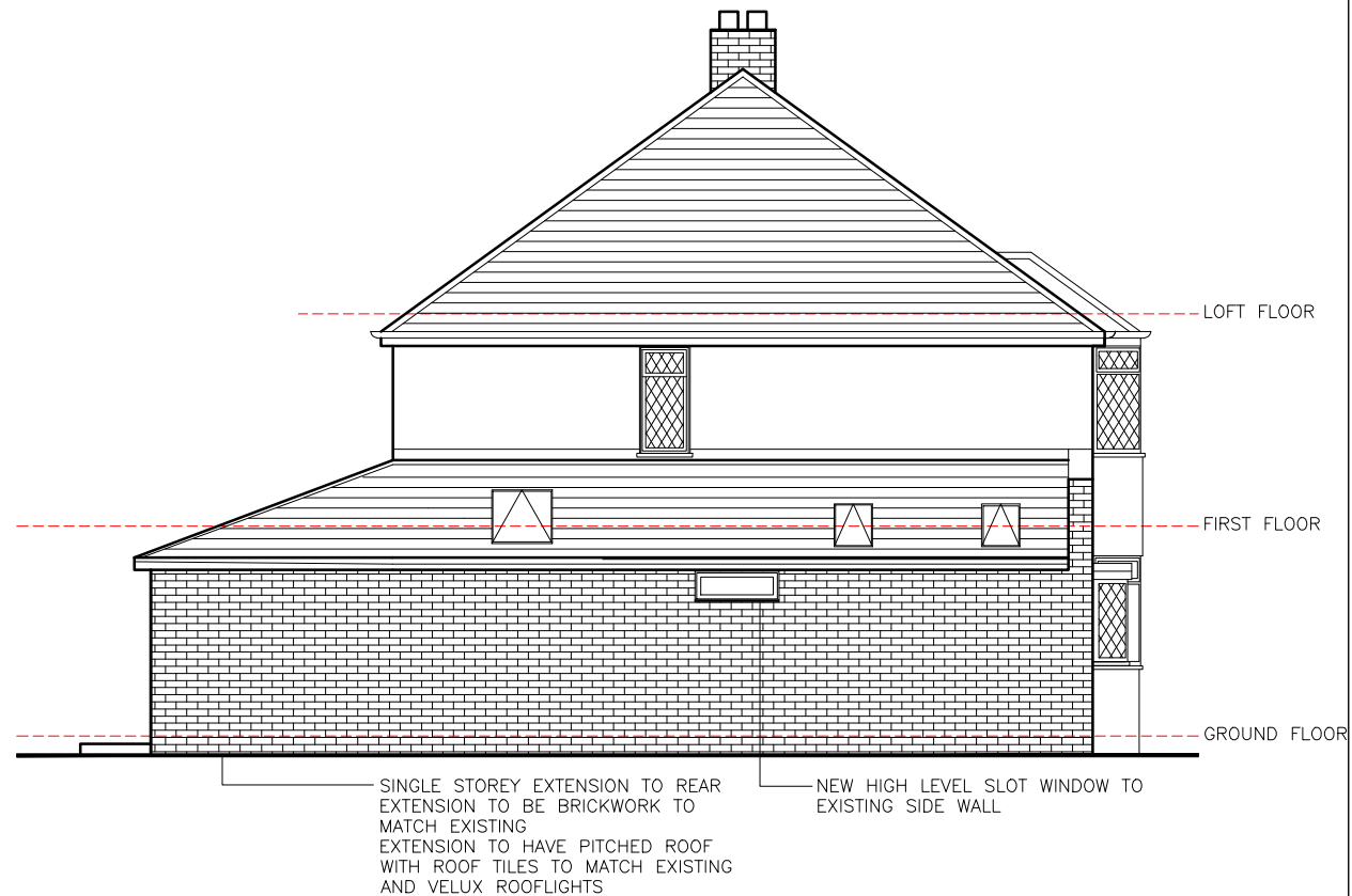
B) Proposed Side Elevation
