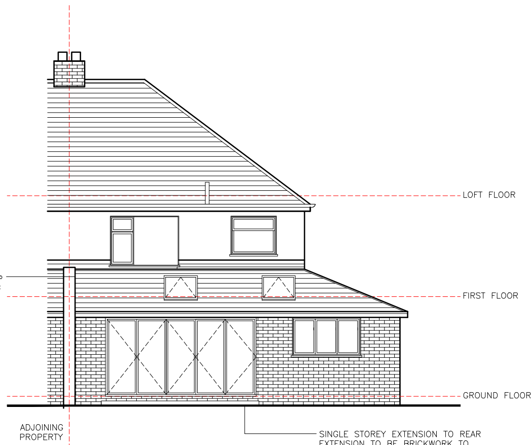
C) Proposed Rear Elevation
