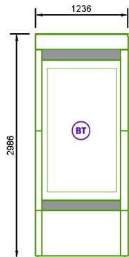
FRONT ELEVATION SCALE 1:50
