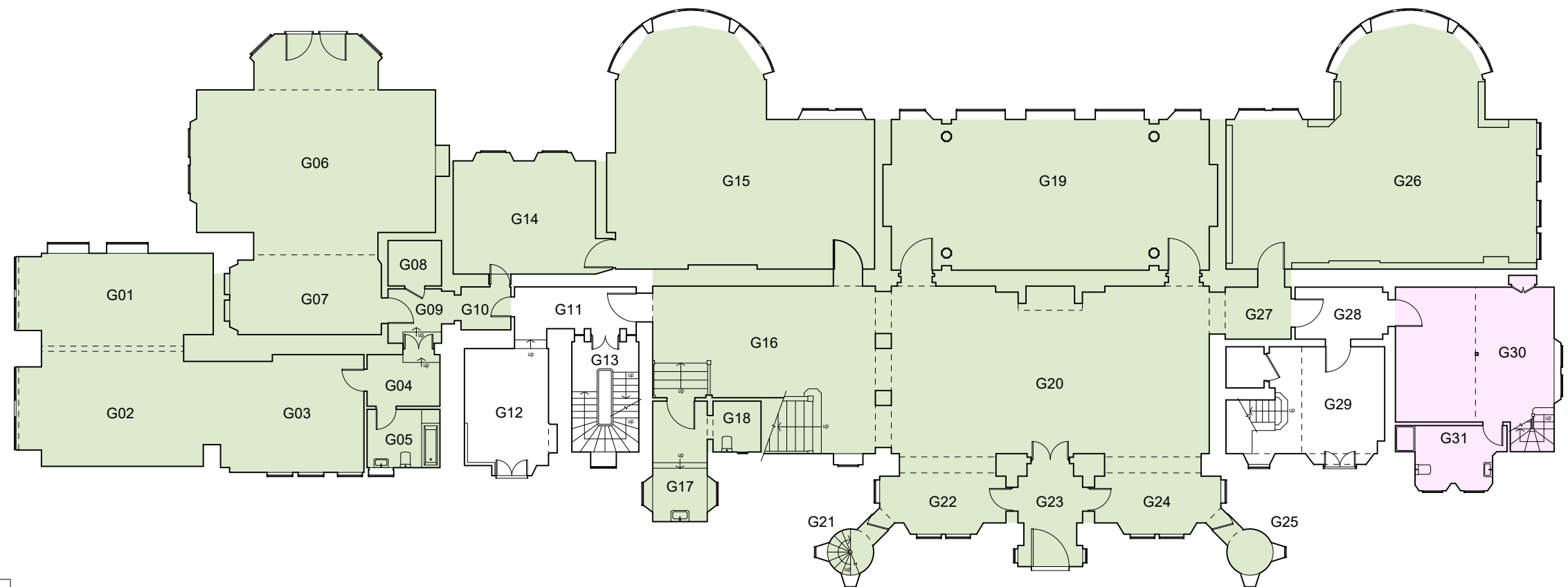
2.04 Layout of flats 1970s ground floor plan
