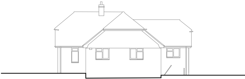
Existing - East Elevation
