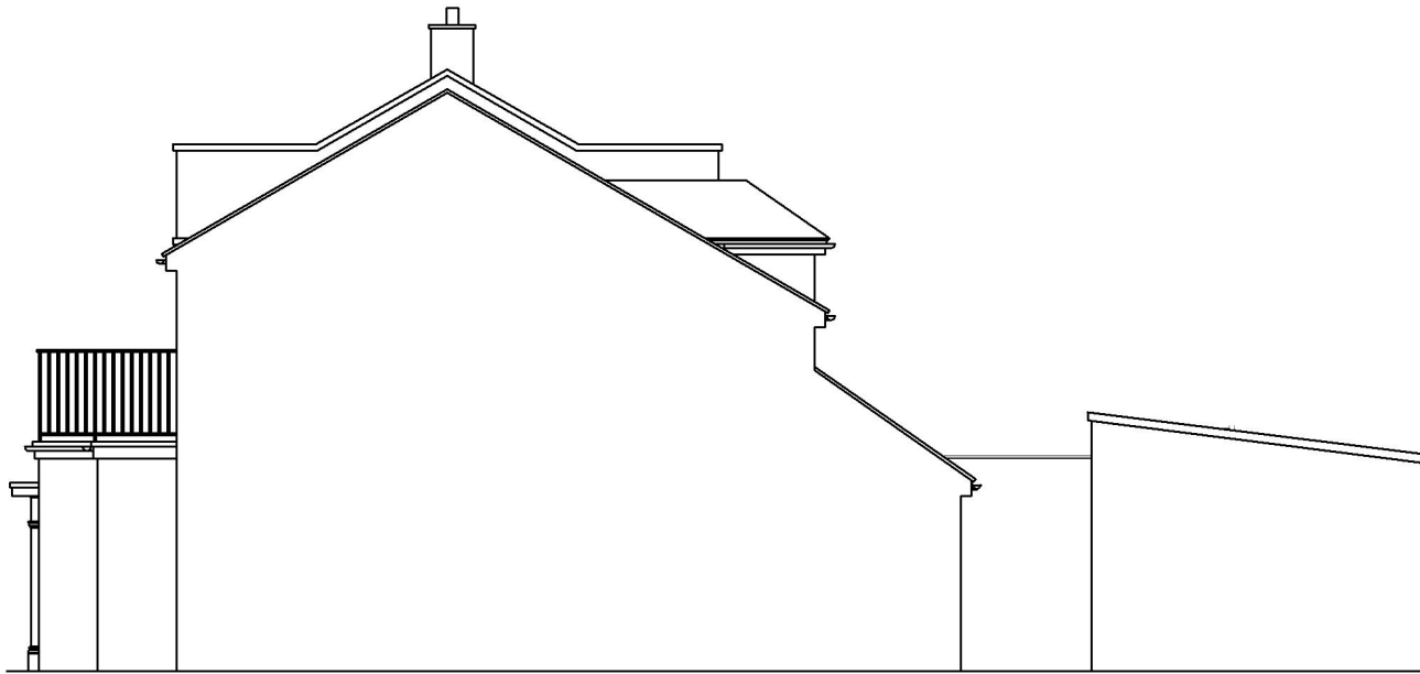
Side Elevation 1:100
