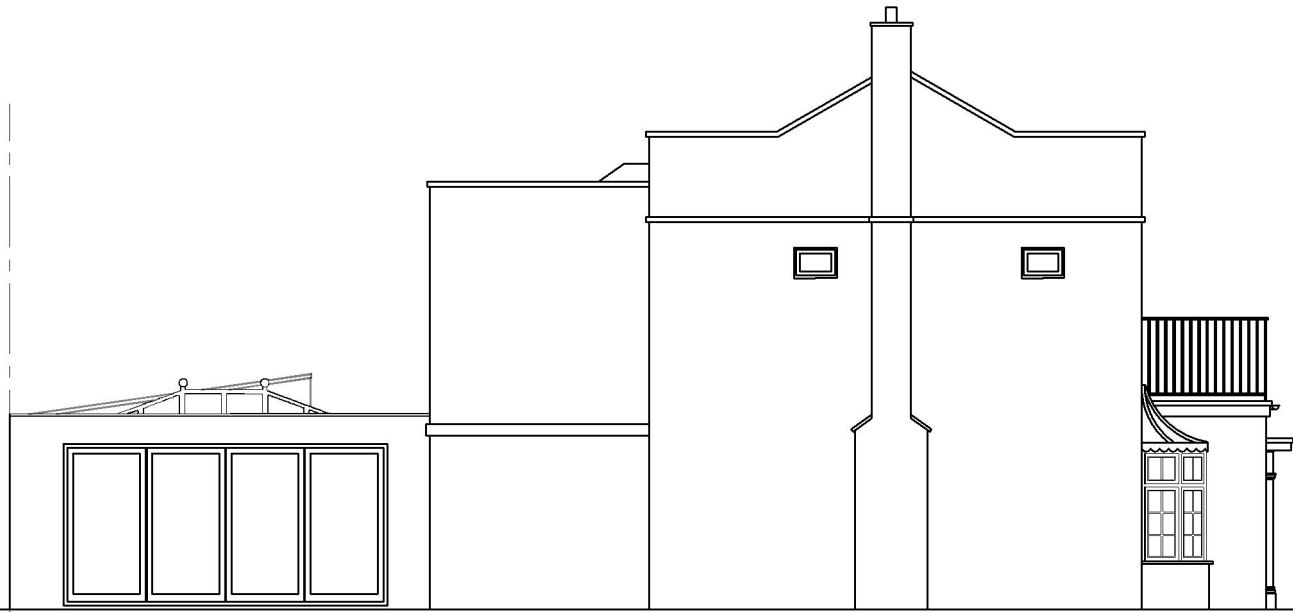
Side Elevation 1:100
