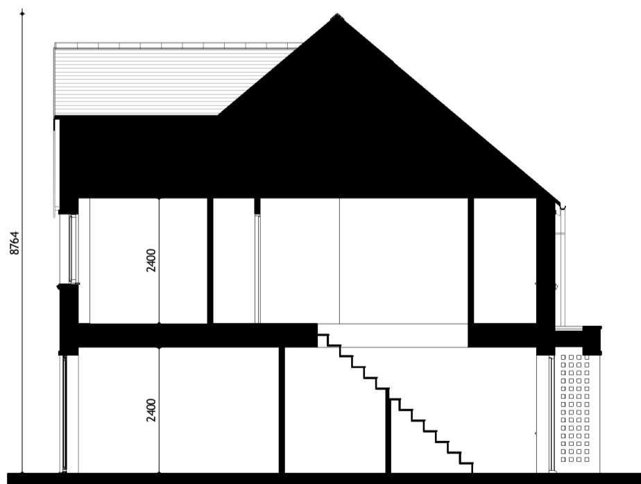
Building Section
