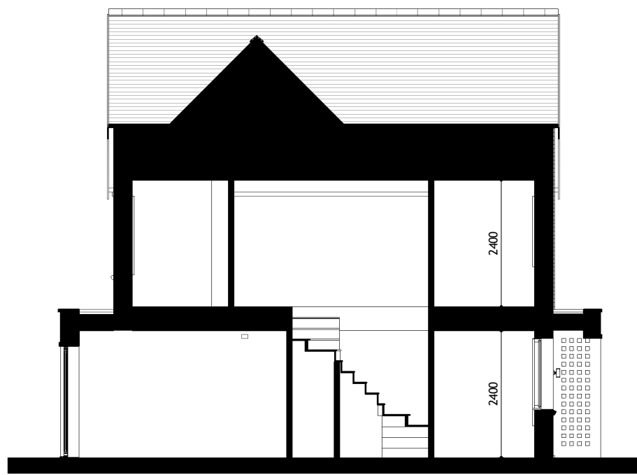
Building Section
