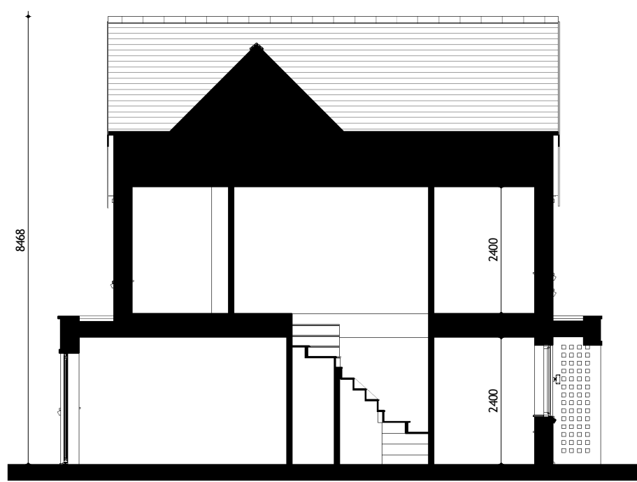
Building Section
