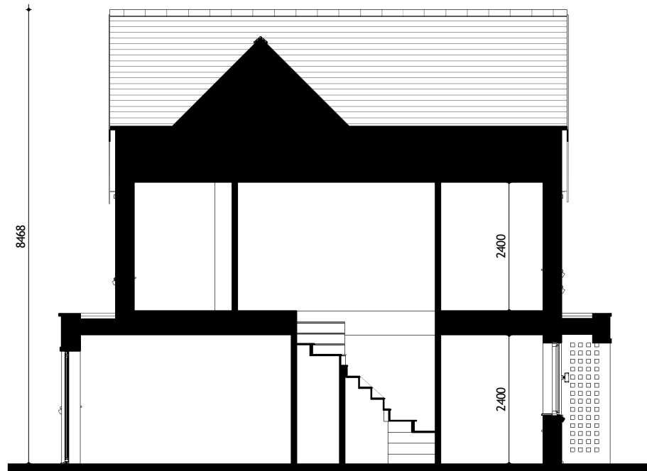
Building Section
