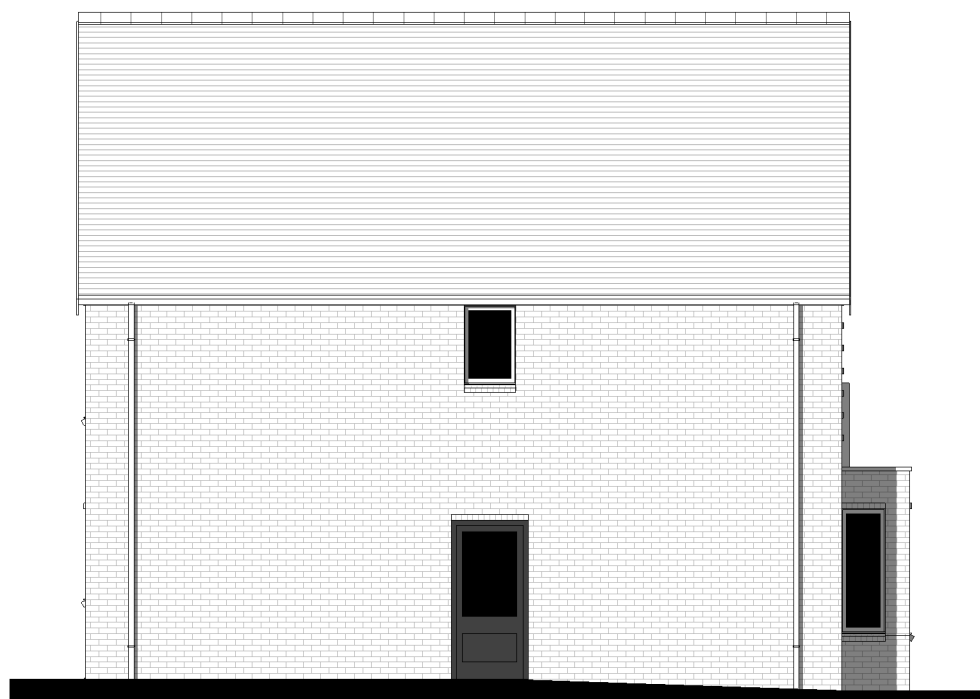
Rear Elevation
