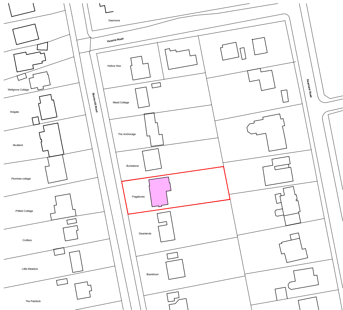
SITE LOCATION PLAN Scale 1:1250 at A1 0m 25m 50m
