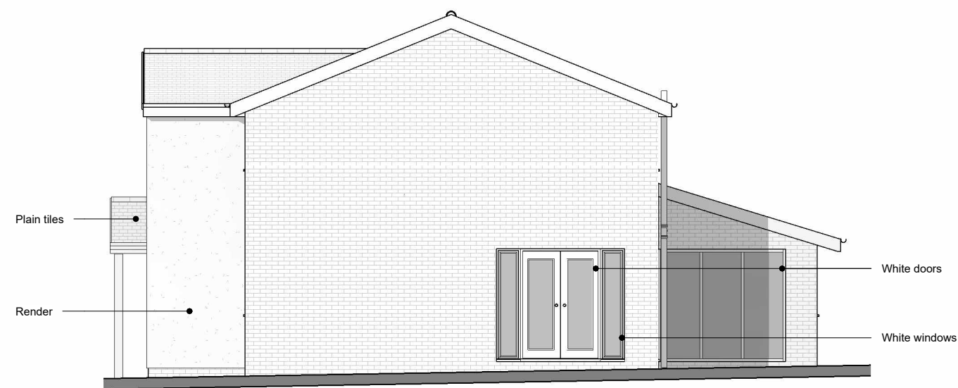
Side 1 Elevation
