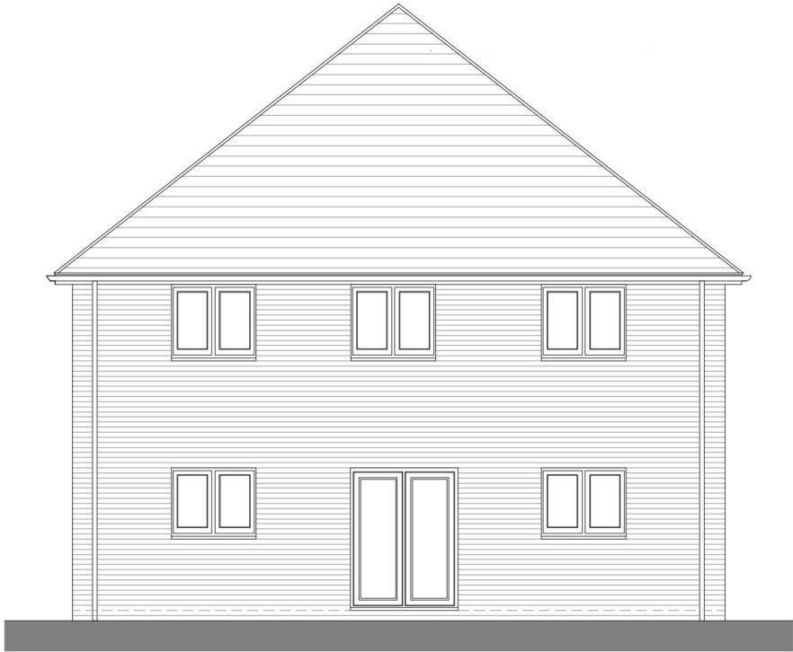
Rear Elevation
