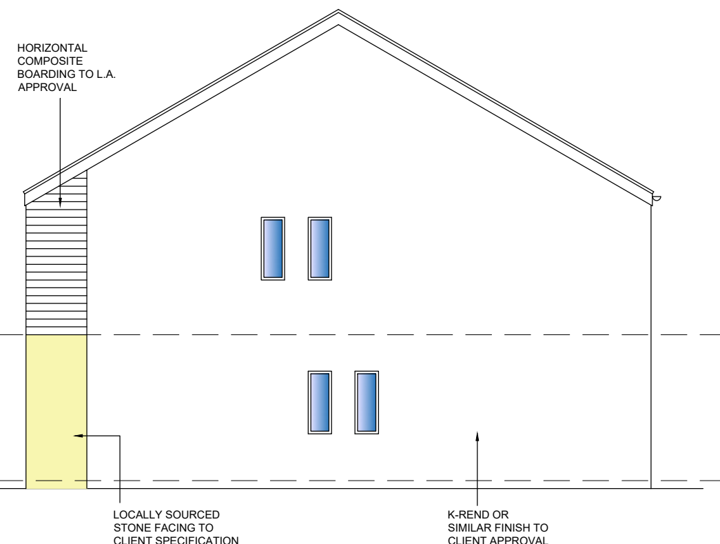
PLOT ONE PROPOSED SIDE ELEVATION
