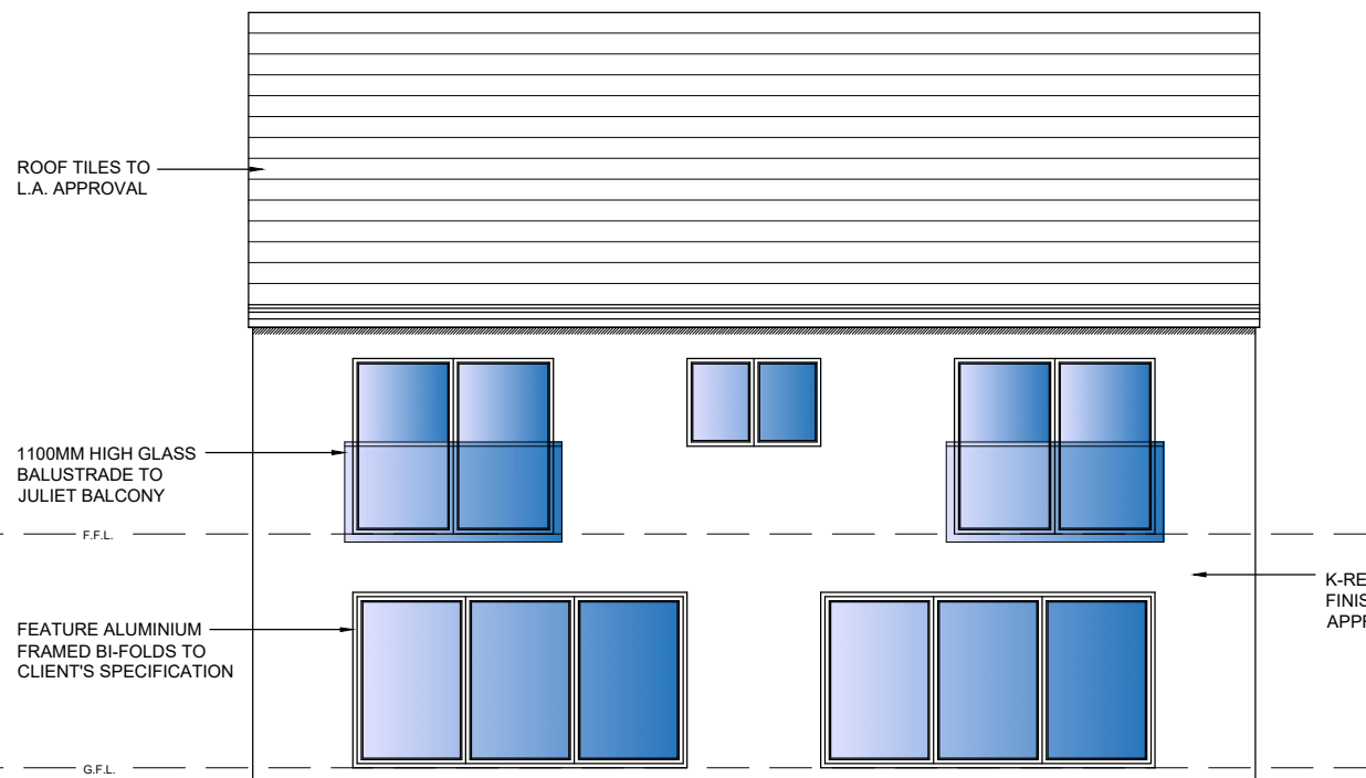
PLOT ONE PROPOSED REAR ELEVATION
