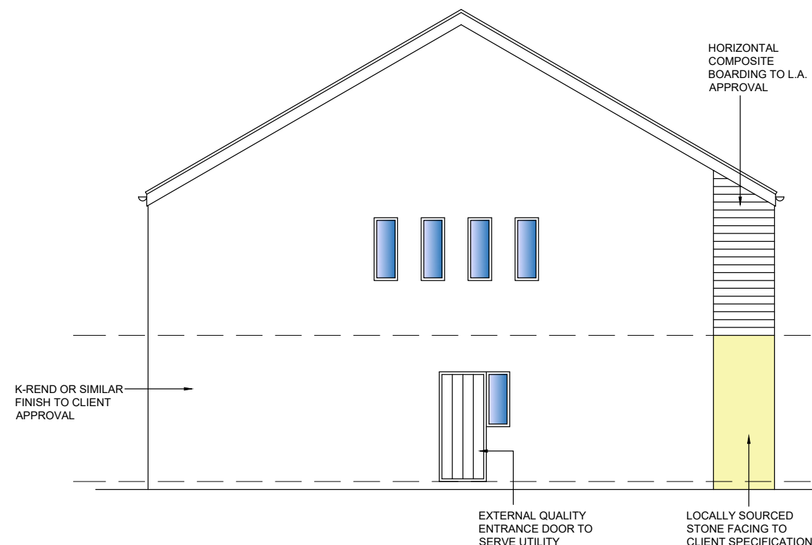
PLOT ONE PROPOSED SIDE ELEVATION
