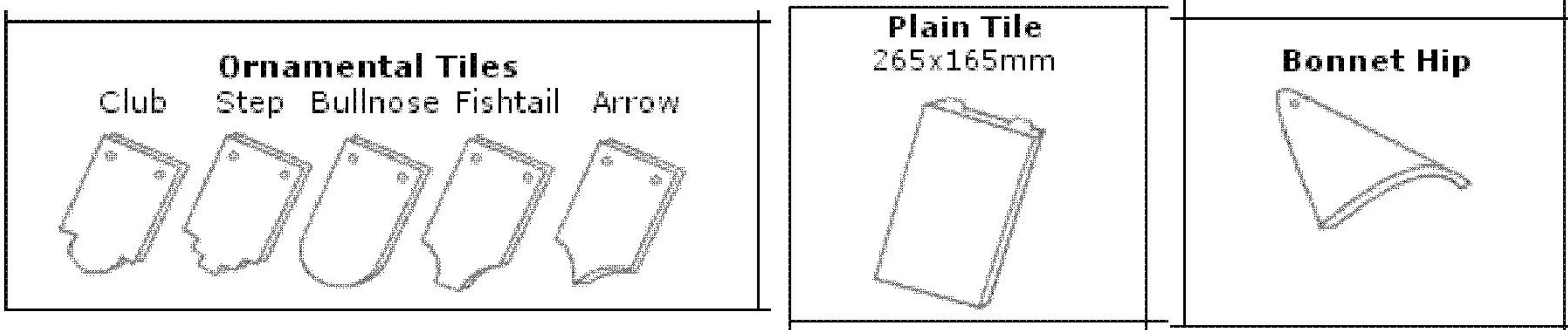
Fig 5: Special and profiled hung and roofing tiles, to match the existing building range, from Aldershaw, or equivalent.
