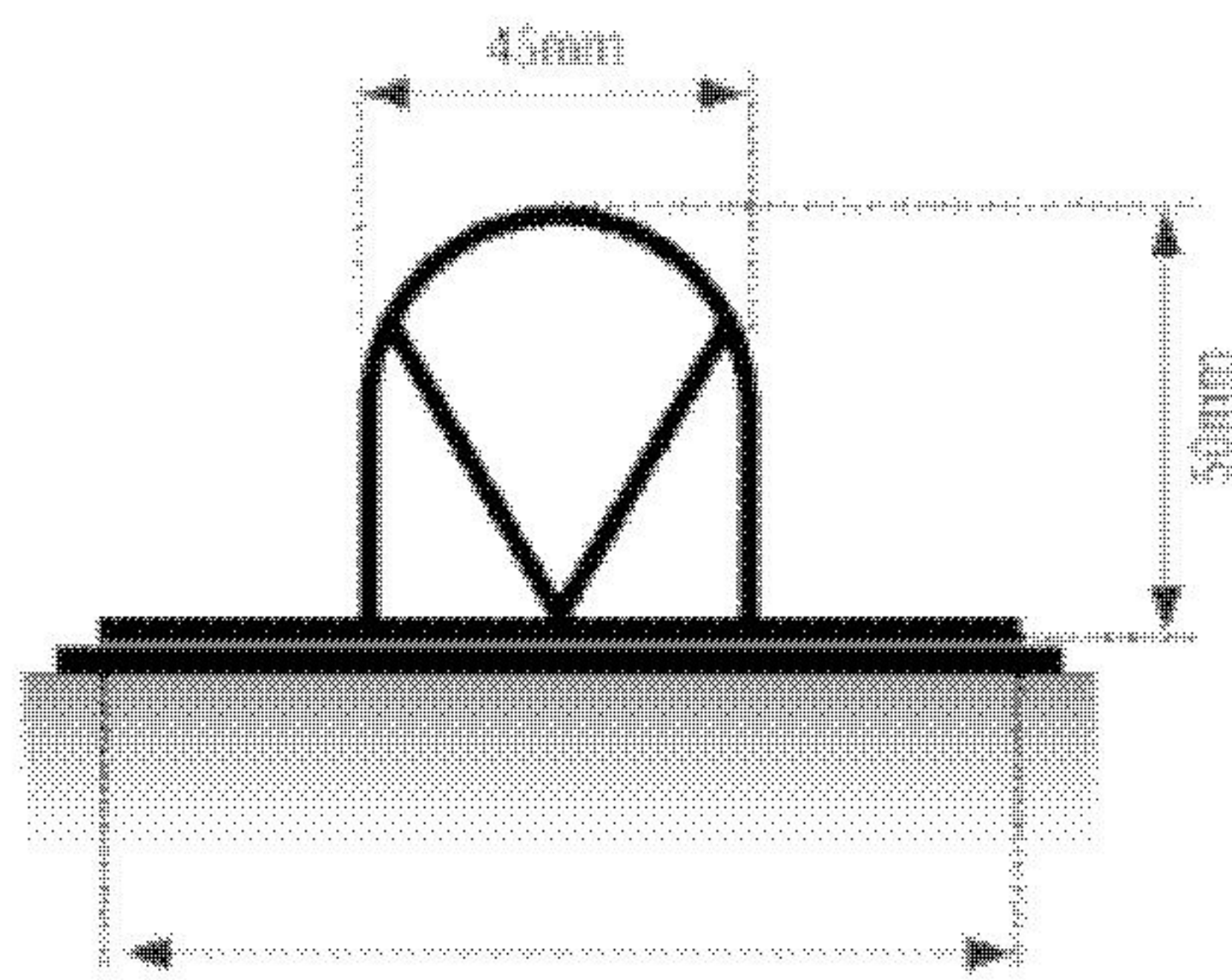
Fig 12: Cross section through Alwitra lead roll effect applied detail, as shown in Figure 11.
