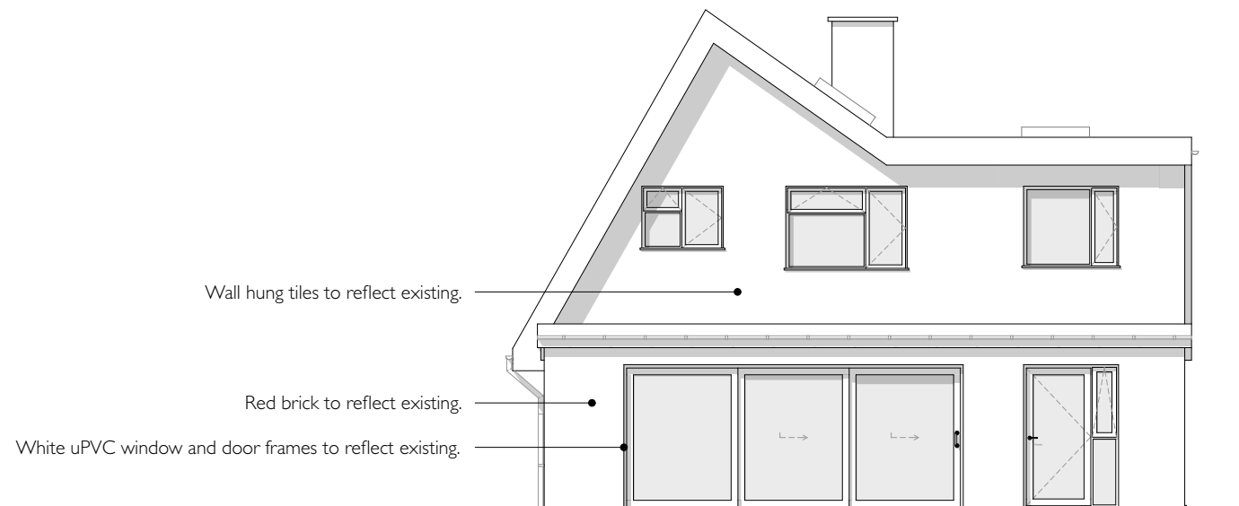
Proposed Rear (West) Elevation Scale 1:100 @ A3
