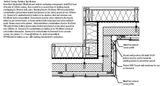
Detail 3 - Cladding External & Internal Corner Junctions (Vertical Cladding) (Houses)
