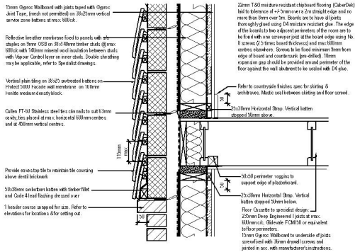
Detail 1 - Floor / External wall Junction & Tile Hanging Termination Detail (Tile Hanging) (Houses)
