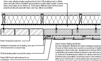
Detail 2 - Brick & Vertical Cladding Junction Detail (Houses)
