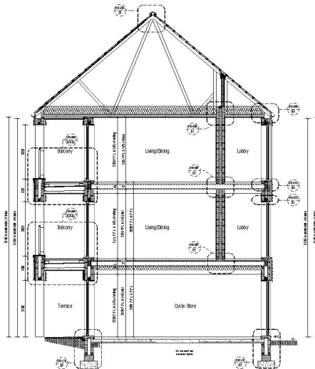
Apartment Block 08 Section B:B Scale 1:50
