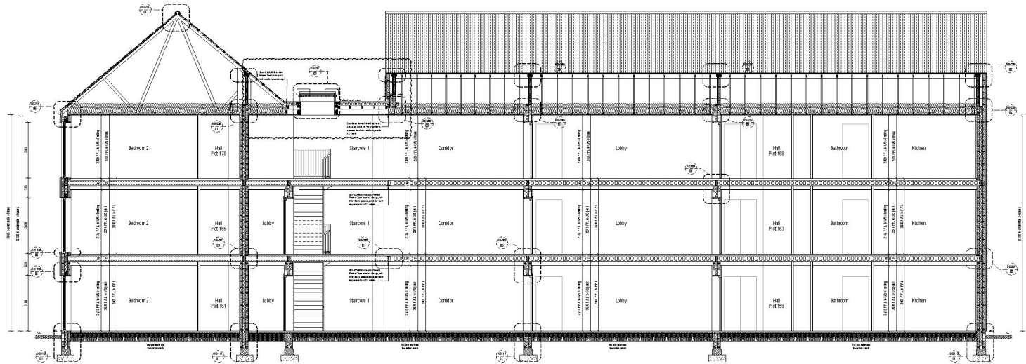
Apartment Block 08 Section A:A Scale 1:50
