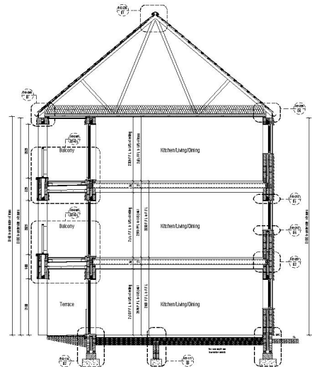
Apartment Block 08 Section C:C Scale 1:50
