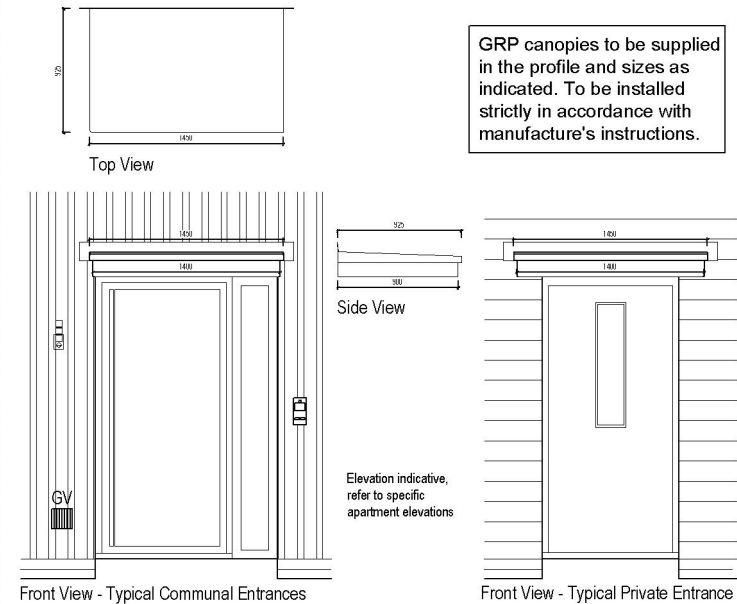
Canopy 4 - Apartment Block 11, 14 - 5no. (4 - Communal & 1 Private) Scale 1:20
