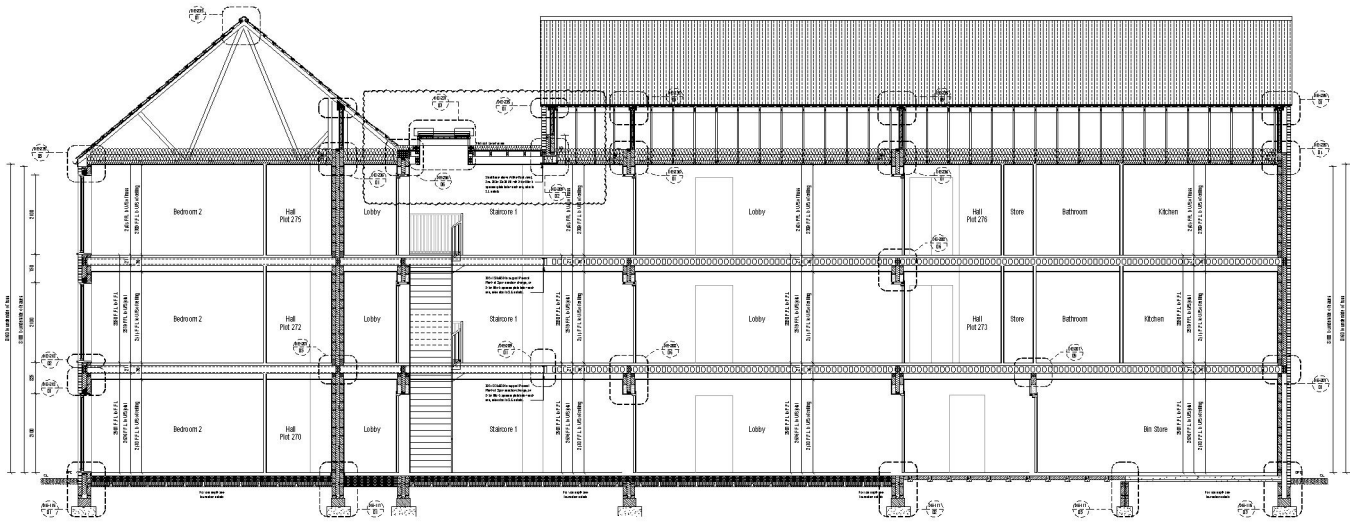
Apartment Block 10 Section A-A Scale 1:50
