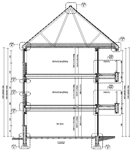
Apartment Block 10 Section E-E Scale 1:50
