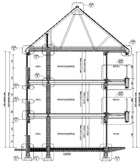
Apartment Block 10 Section D-D Scale 1:50
