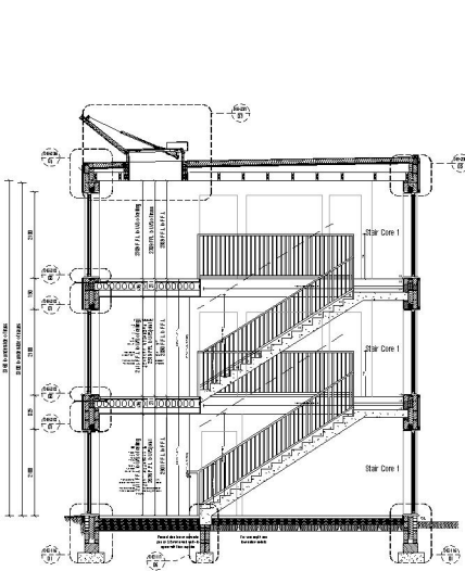
Apartment Block 10 Section C-C Scale 1:50
