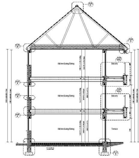
Apartment Block 10 Section B-B Scale 1:50
