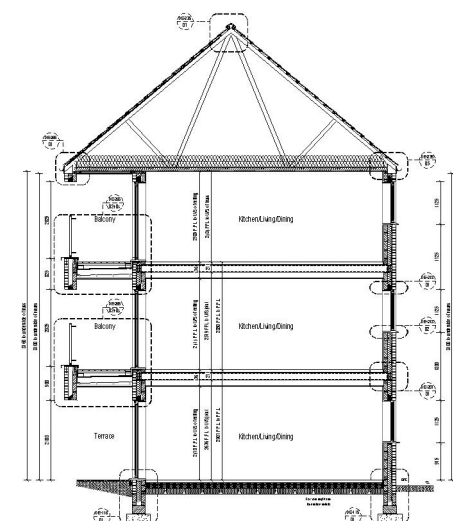
Apartment Block 12 Section C:C Scale 1:50
