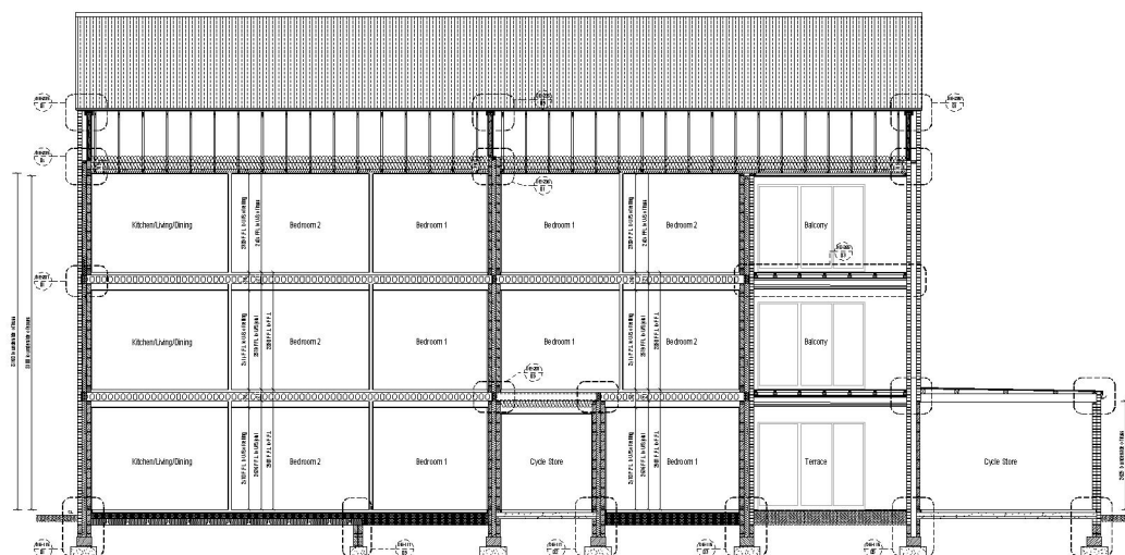
Apartment Block 12 Section E:E Scale 1:50
