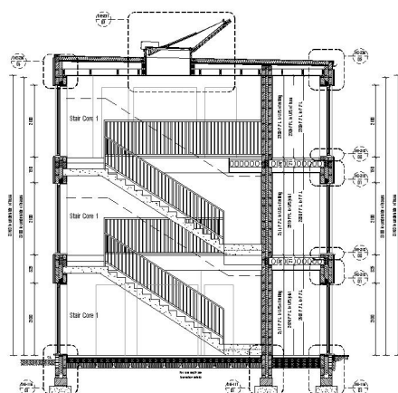
Apartment Block 12 Section D:D Scale 1:50
