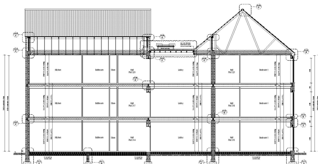
Apartment Block 12 Section A:A Scale 1:50
