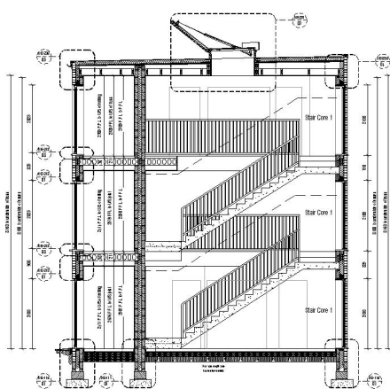
Apartment Block 13 Section C:C Scale 1:50
