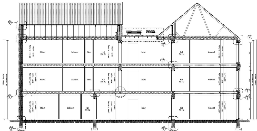
Apartment Block 13 Section A:A Scale 1:50
