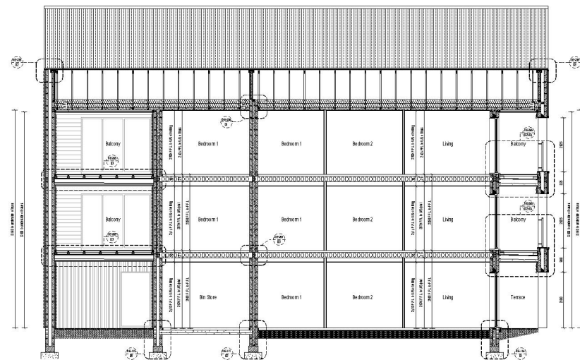
Apartment Block 13 Section D:D Scale 1:50
