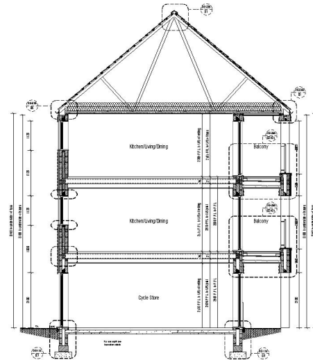
Apartment Block 13 Section B:B Scale 1:50
