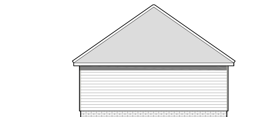
Proposed South Elevation
