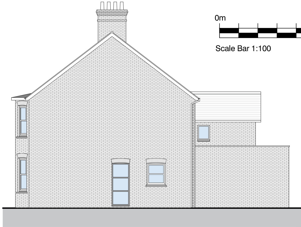
Side Elevation (S) 1:100
