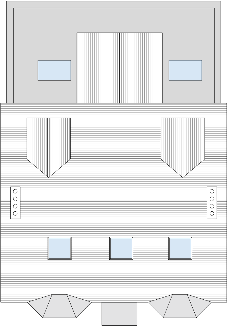
Roof Plan 1:100
