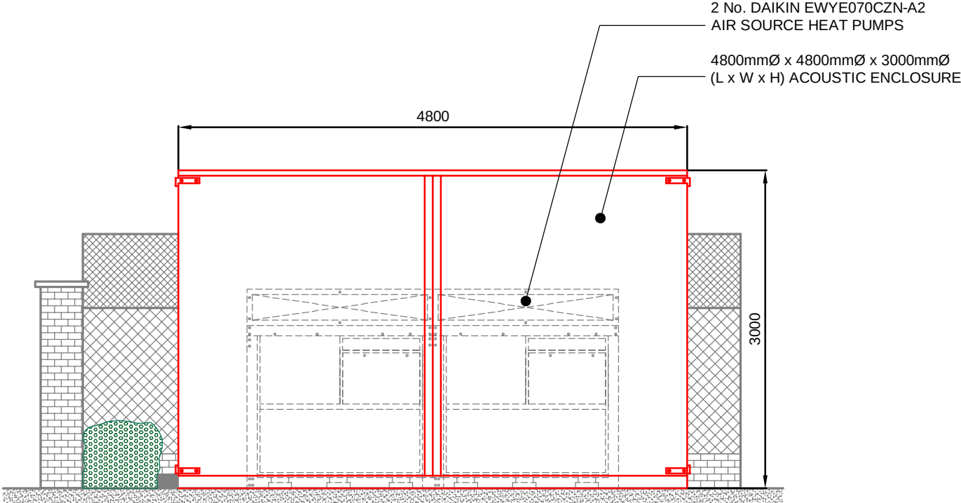
ELEVATION A - PROPOSED ELEVATION OF AIR SOURCE HEAT PUMPS & ACOUSTIC ENCLOSURE (1:50)
