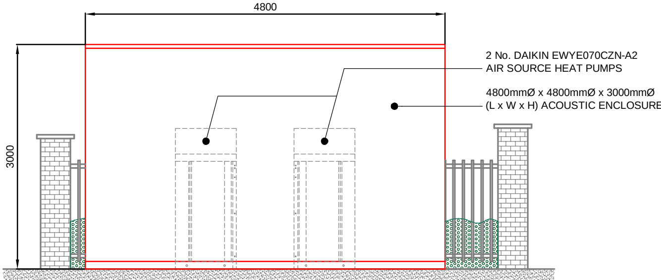
ELEVATION D - PROPOSED ELEVATION OF AIR SOURCE HEAT PUMPS & ACOUSTIC ENCLOSURE (1:50)
