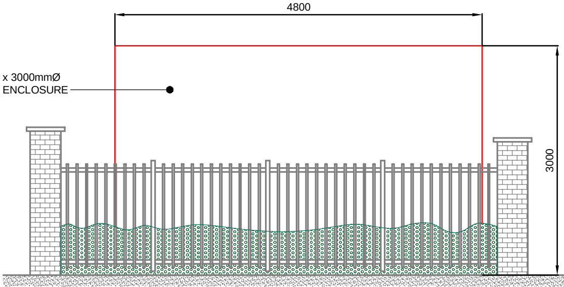
ELEVATION B - PROPOSED ELEVATION OF AIR SOURCE HEAT PUMPS & ACOUSTIC ENCLOSURE (1:50)
