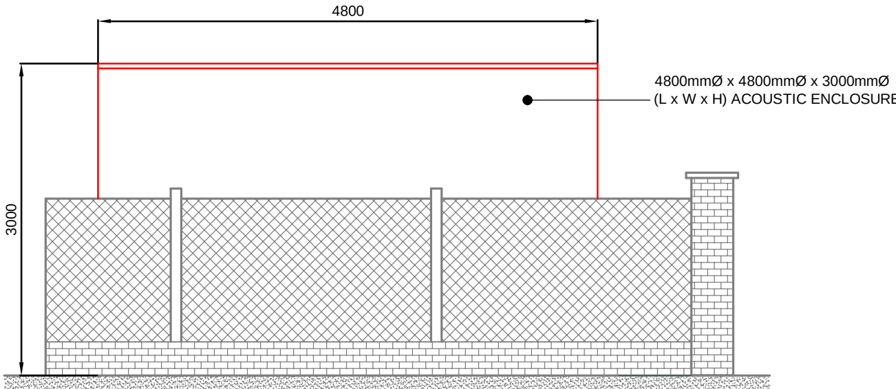
ELEVATION C - PROPOSED ELEVATION OF AIR SOURCE HEAT PUMPS & ACOUSTIC ENCLOSURE (1:50)
