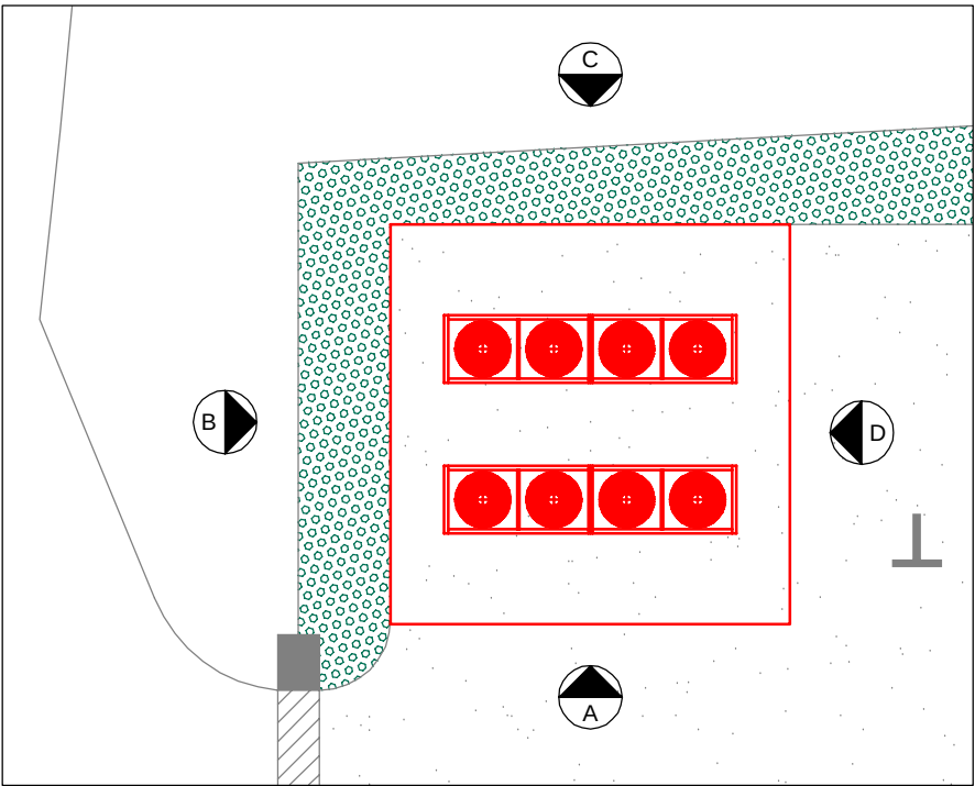
INDICATIVE AIR SOURCE HEAT PUMP ARRANGEMENT (1:100)
