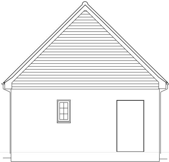
NORTH ELEVATION
