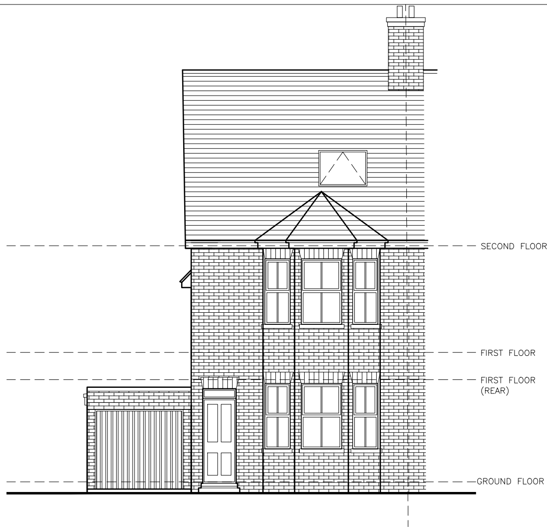
A) Existing Front Elevation
