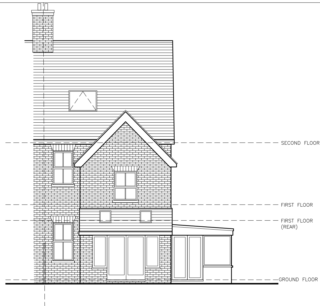
B) Existing Rear Elevation
