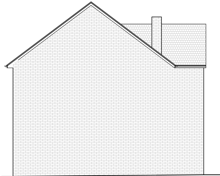
EXISTING SIDE ELEVATION FROM No.23
