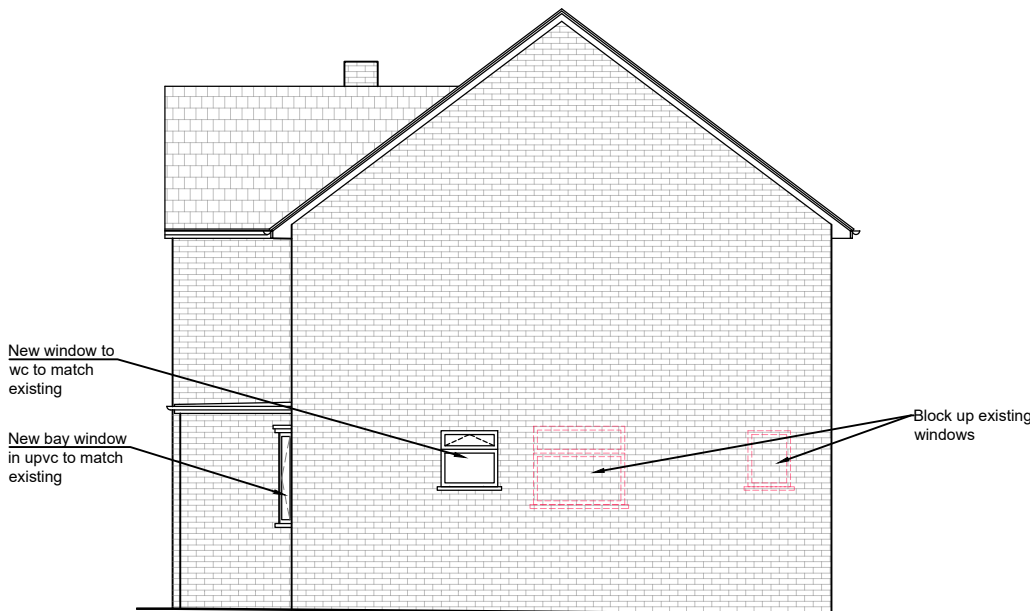
PROPOSED SIDE ELEVATION FROM No.27
