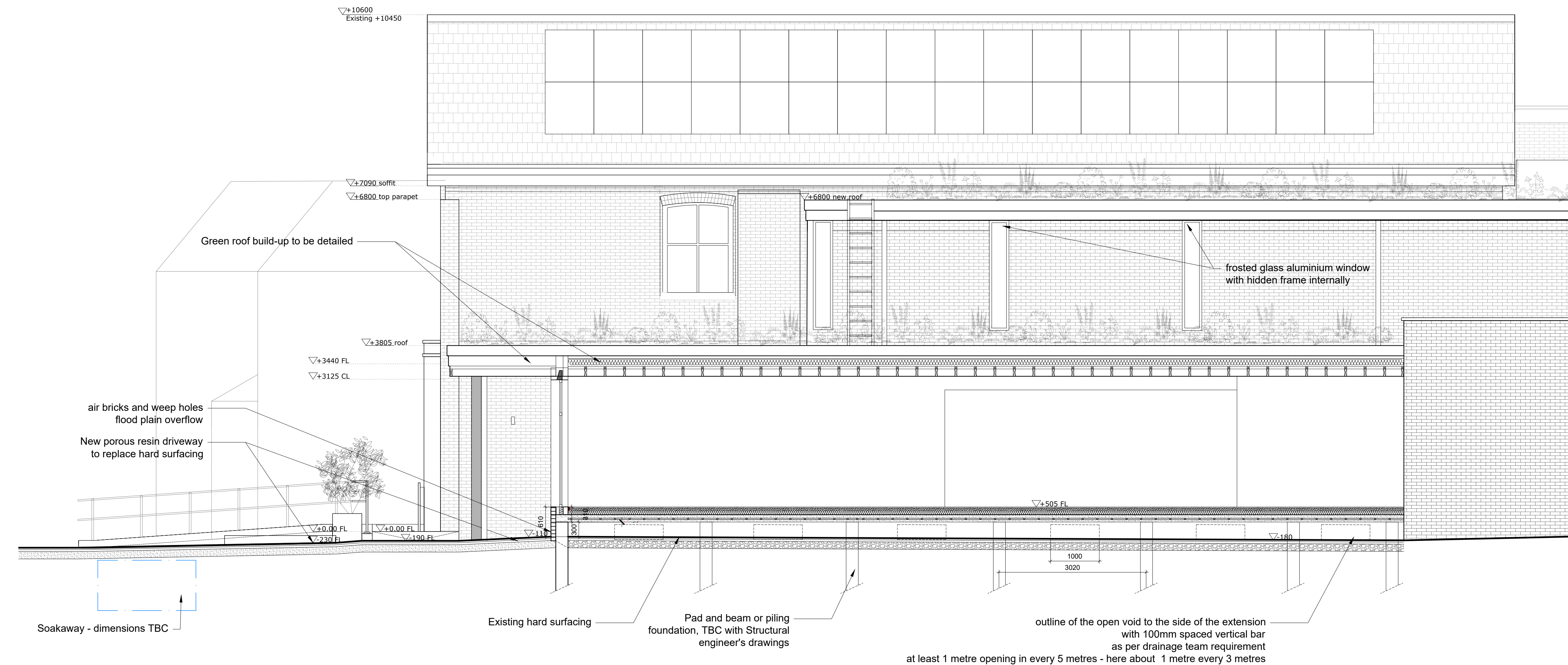
South (Front) Elevation 1:100
