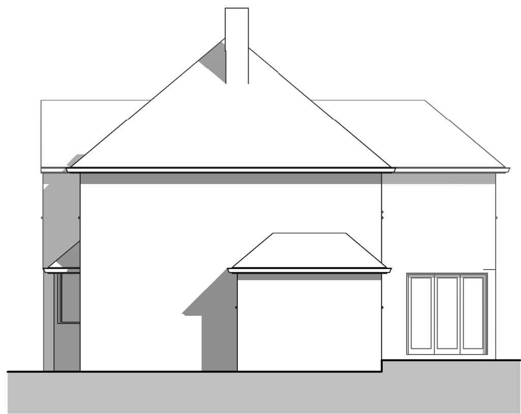
5 Existing West Elevation 1 : 100
