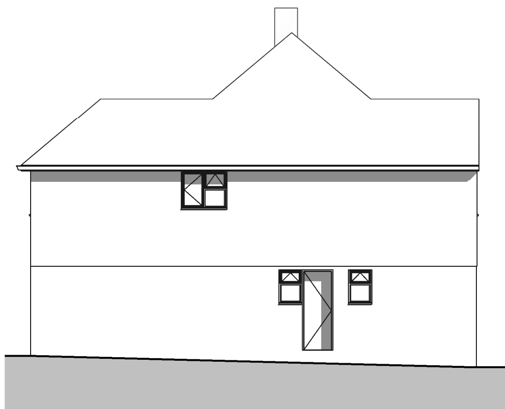
7 Existing East Elevation 1 : 100
