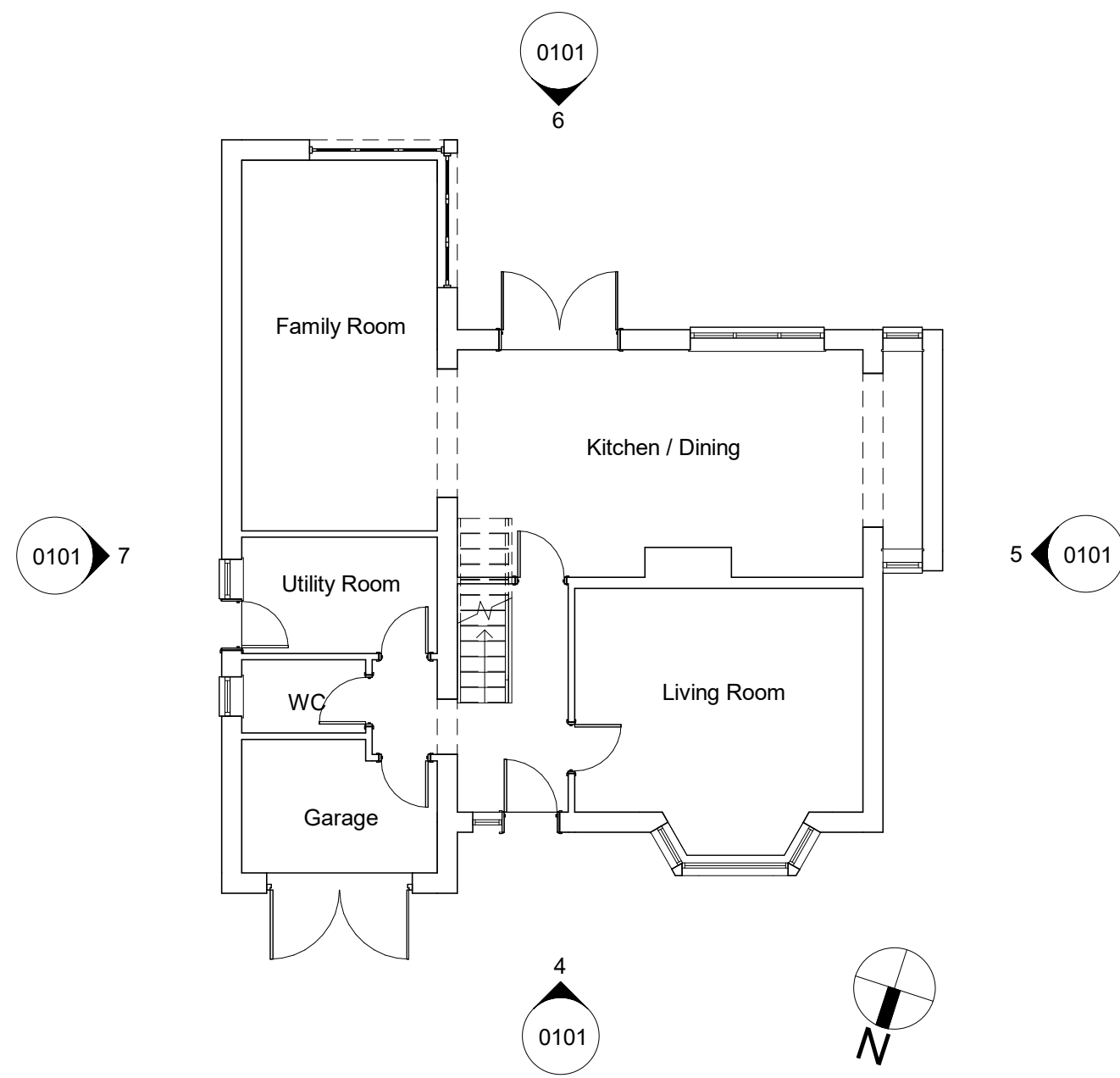
1 Existing - L0 Ground Floor 1 : 100
