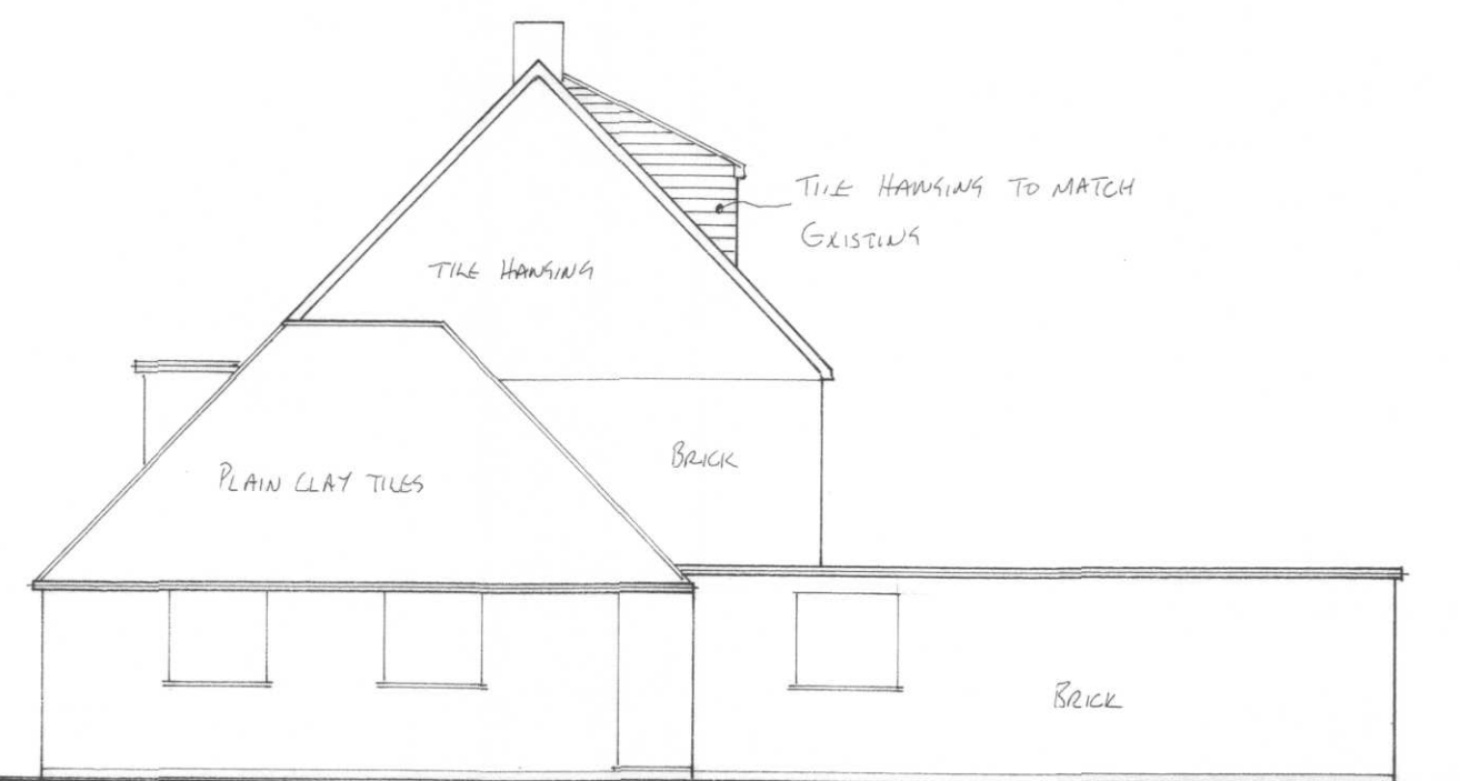
SIDE ELEVATION (NORTH)
