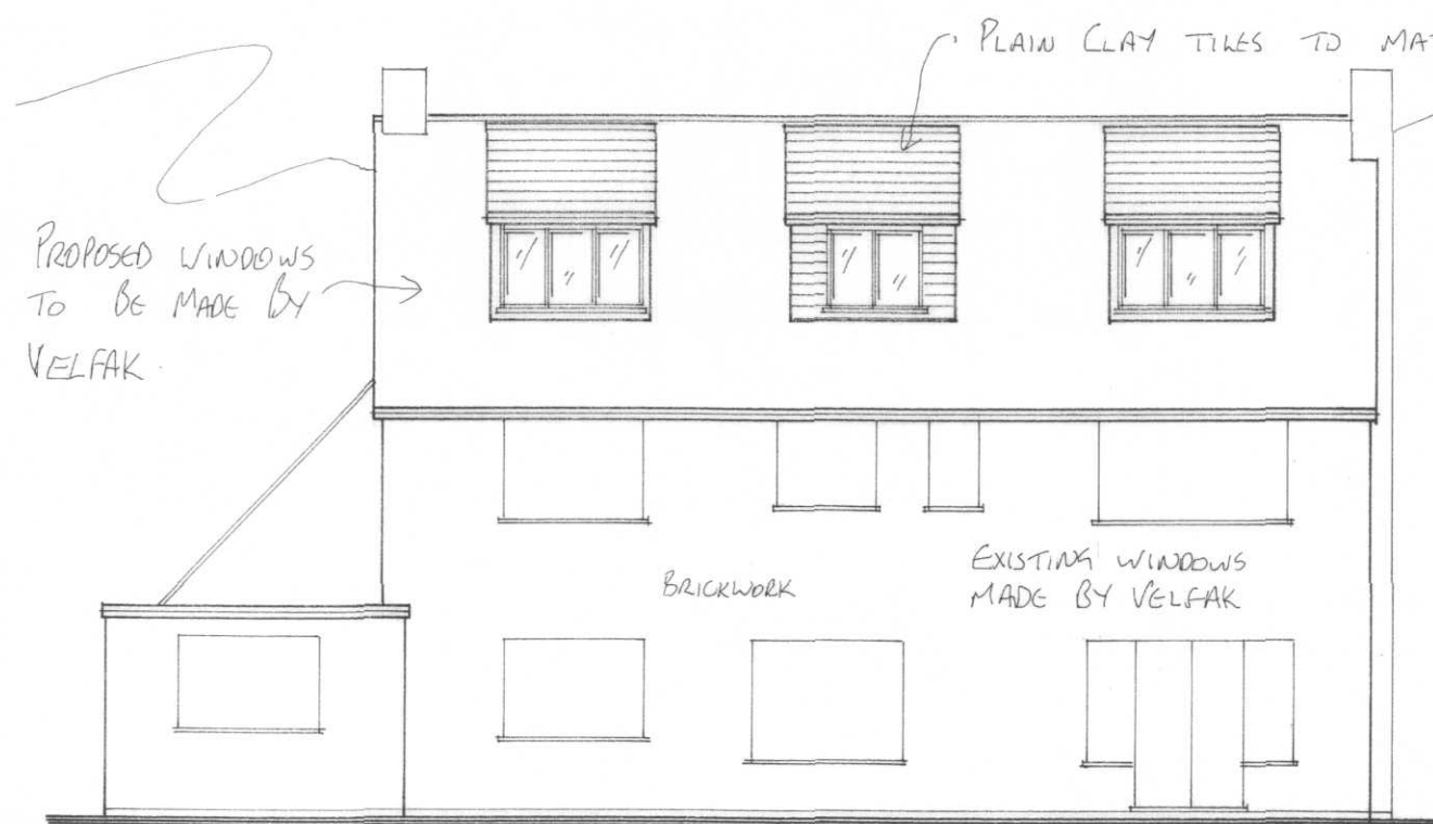
REAR ELEVATION
