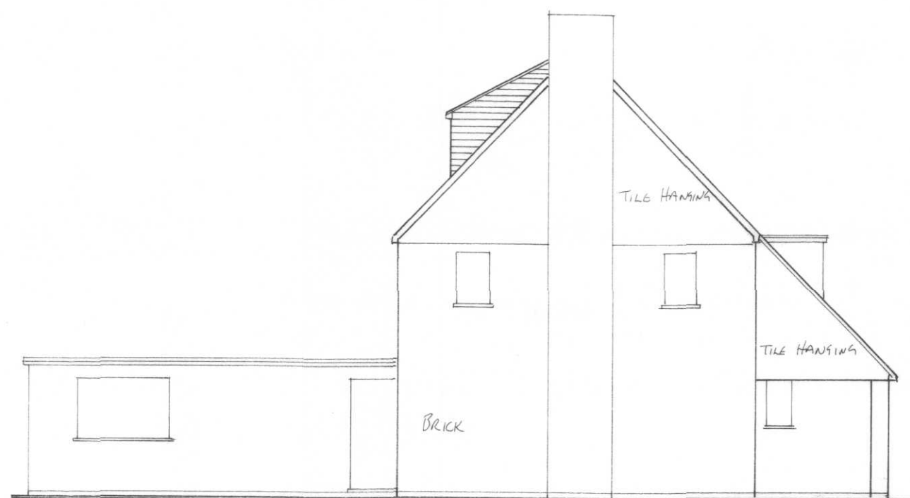
SIDE ELEVATION (SOUTH)
